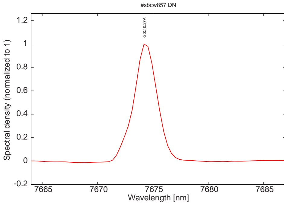
Figure 9: monomode spectrum at -20C and 0.27A
