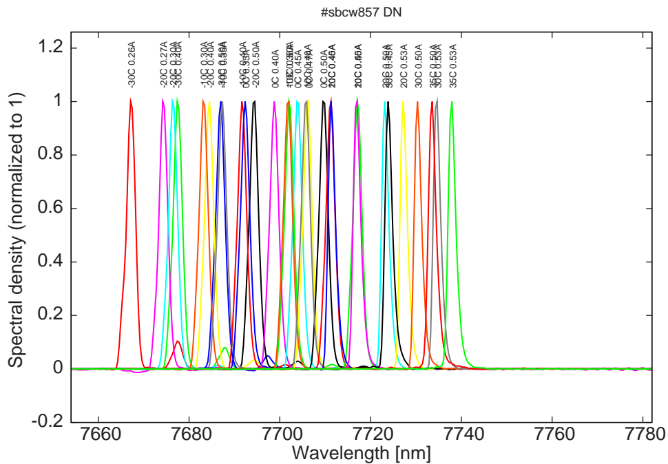
Figure 6: spectra at -30C, -20C, -10C, 0C, 10C, 20C, 30C and 35C for various DC currents
