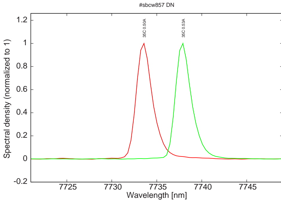
Figure 17: spectra at 35C for various DC currents (all monomode)
