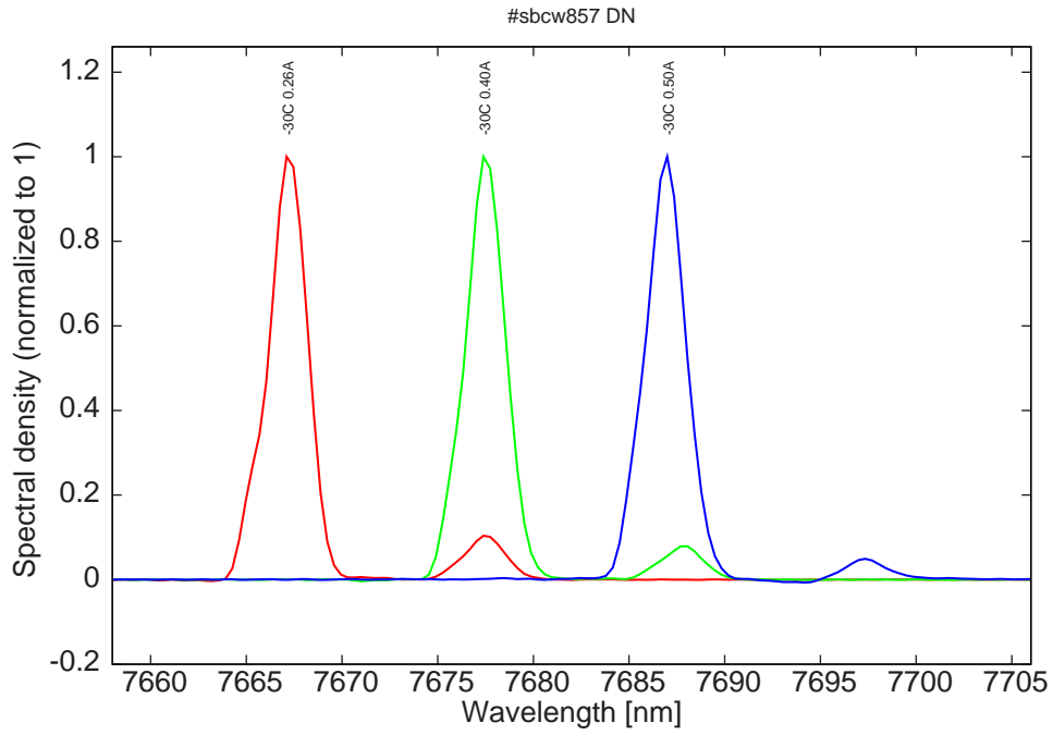
Figure 7: spectra at -30C for various DC currents (all bimode)
