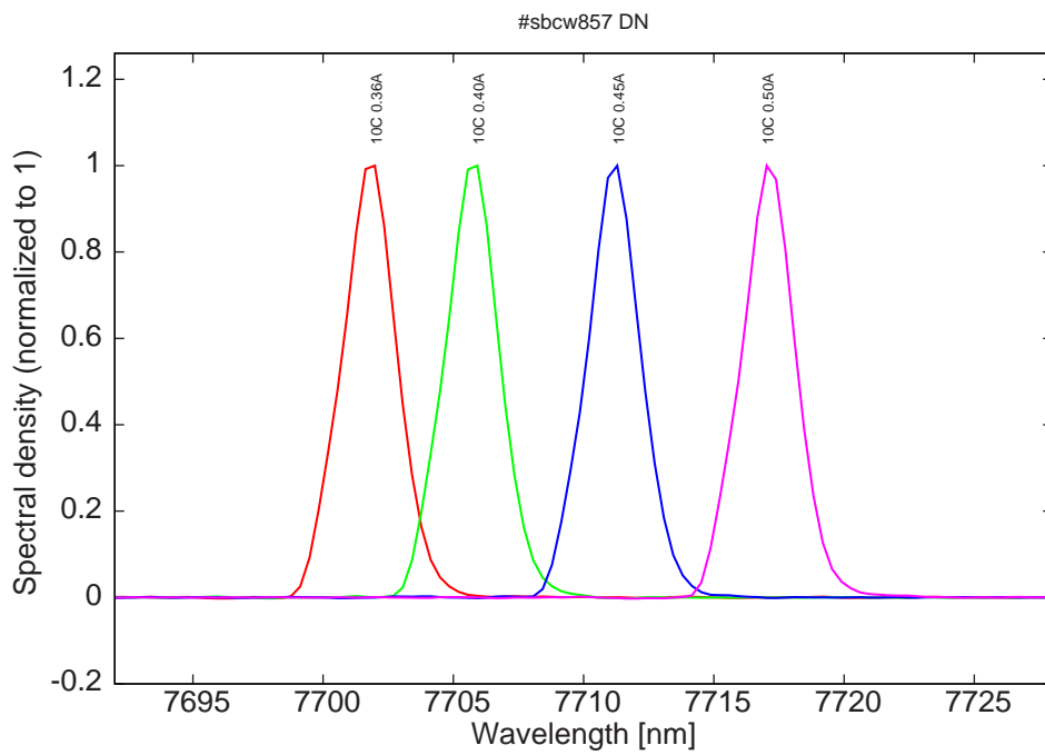
Figure 14: spectra at 10C for various DC currents (all monomode)
