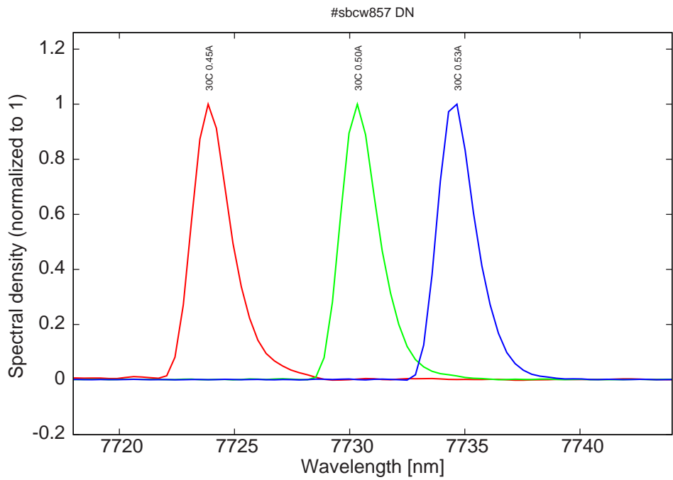
Figure 16: spectra at 30C for various DC currents (all monomode)
