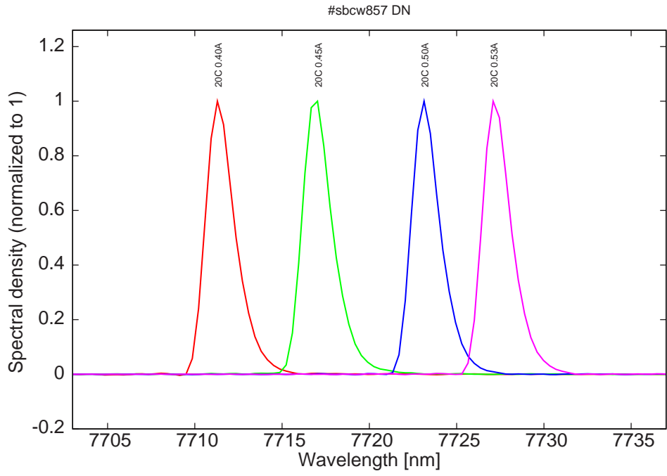
Figure 15: spectra at 20C for various DC currents (all monomode)
