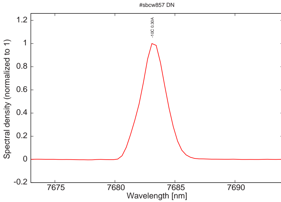
Figure 11: monomode spectrum at -10C and 0.30A
