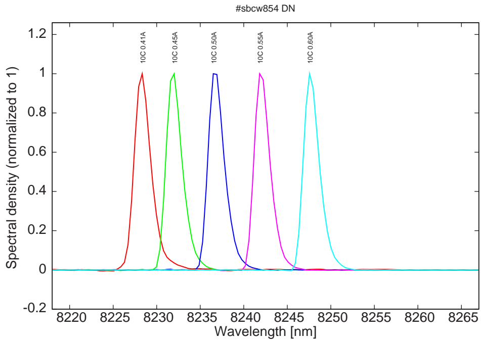
Figure 12: spectra at 10C for various DC currents
