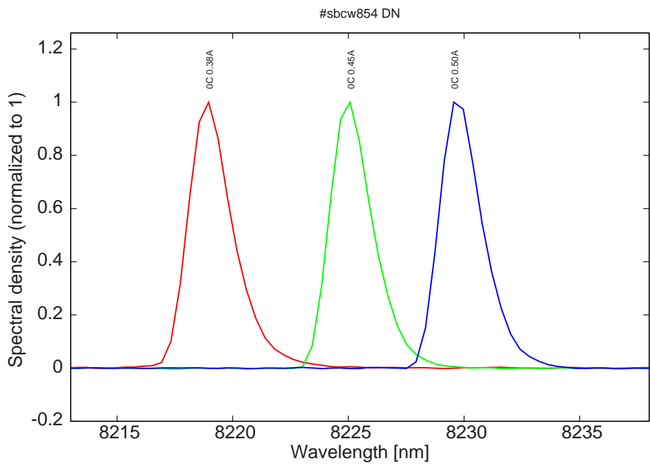
Figure 11: spectra at 0C for various DC currents
