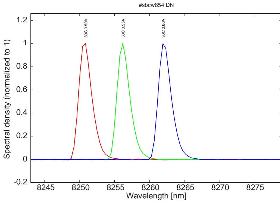
Figure 14: spectra at 30C for various DC currents
