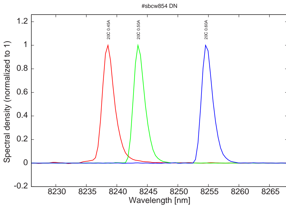
Figure 13: spectra at 20C for various DC currents
