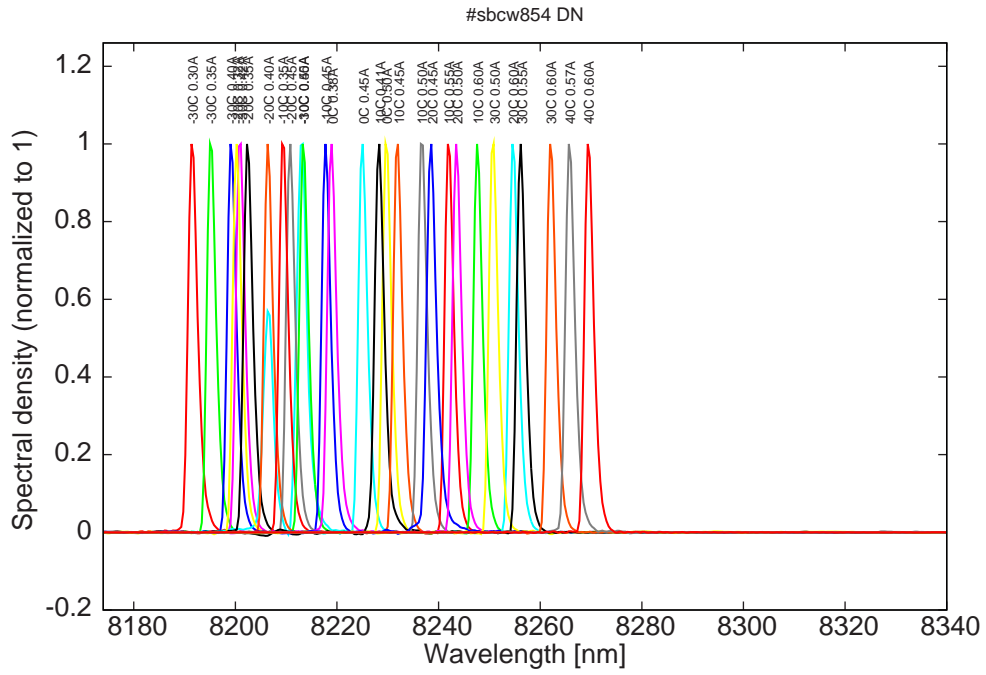
Figure 6: spectra at -30C, -20C, -10C, 0C, 10C, 20C, 30C, 40C and 45C for various DC currents
