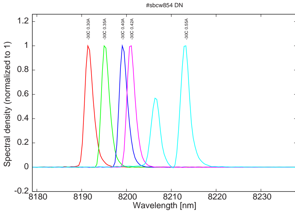
Figure 7: spectra at -30C for various DC currents (monomode up to 0.42A)
