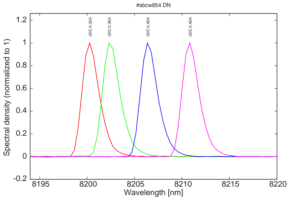
Figure 9: spectra at -20C for various DC currents (monomode up to 0.45A)
