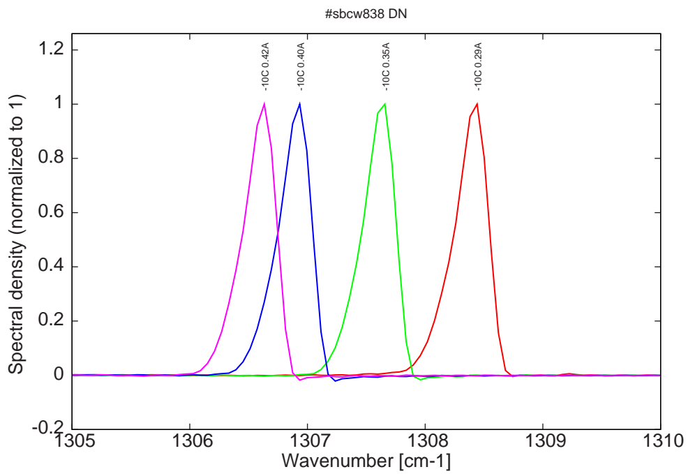
Figure 11: spectra at -10C for various DC currents (monomode range, up to 0.42A)
