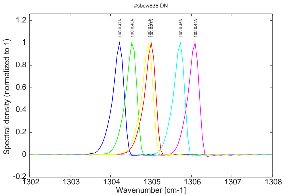
Figure 15: spectra at 10C for various DC currents (monomode range, with mode jumping for I > 0.42A , see Fig.3)
