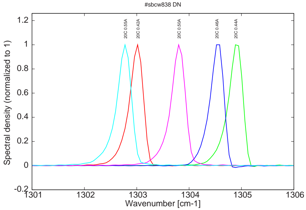
Figure 16: spectra at 20C for various DC currents (all monomode, with mode jumping for I > 0.42A , see Fig.3)
