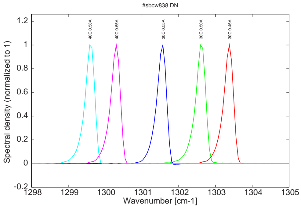
Figure 17: spectra at 30C and 40C for various DC currents (all monomode, but on another mode compared to lower temperatures, see Fig.3)
