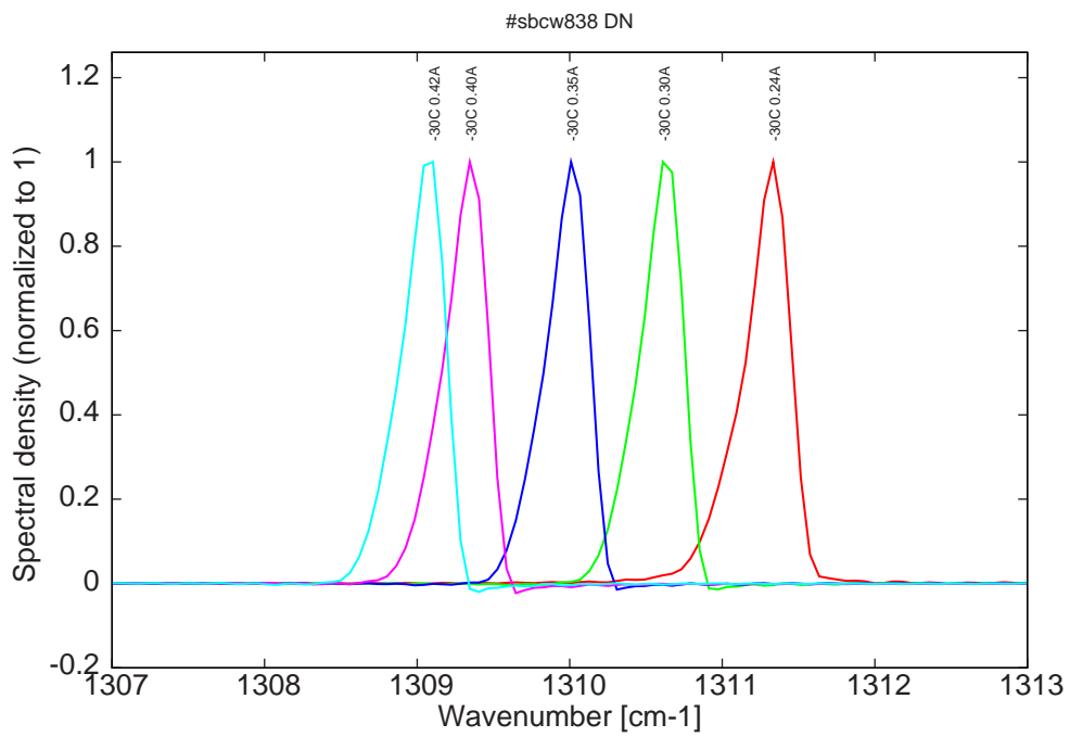
Figure 7: spectra at -30C for various DC currents (monomode range, up to 0.42A)
