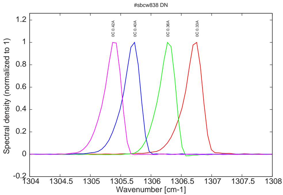
Figure 13: spectra at 0C for various DC currents (monomode range, up to 0.42A)
