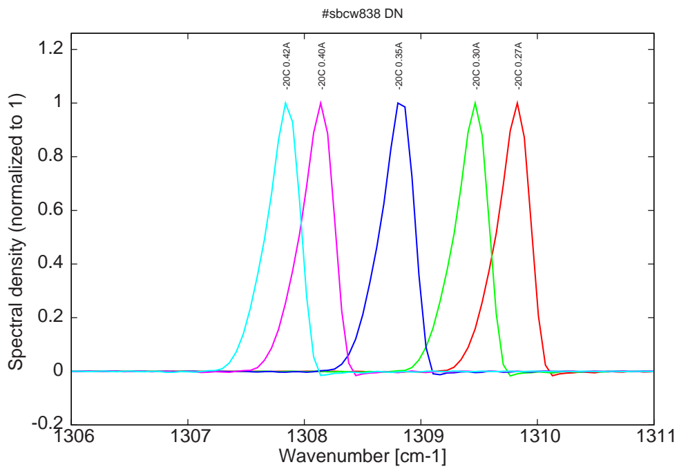
Figure 9: spectra at -20C for various DC currents (monomode range, up to 0.42A)
