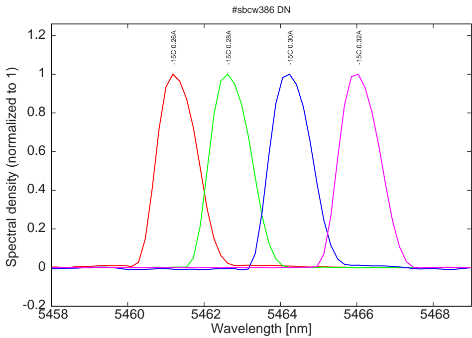
Figure 8: spectra at -15C for various DC currents
