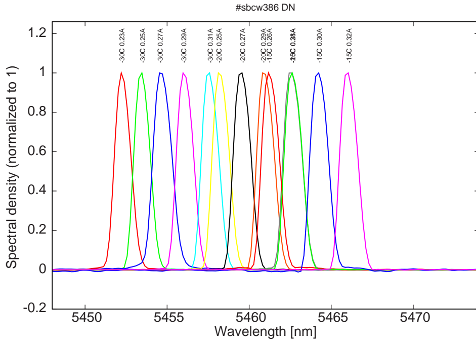
Figure 5: spectra at -30C, -20C and -15C for various DC currents
