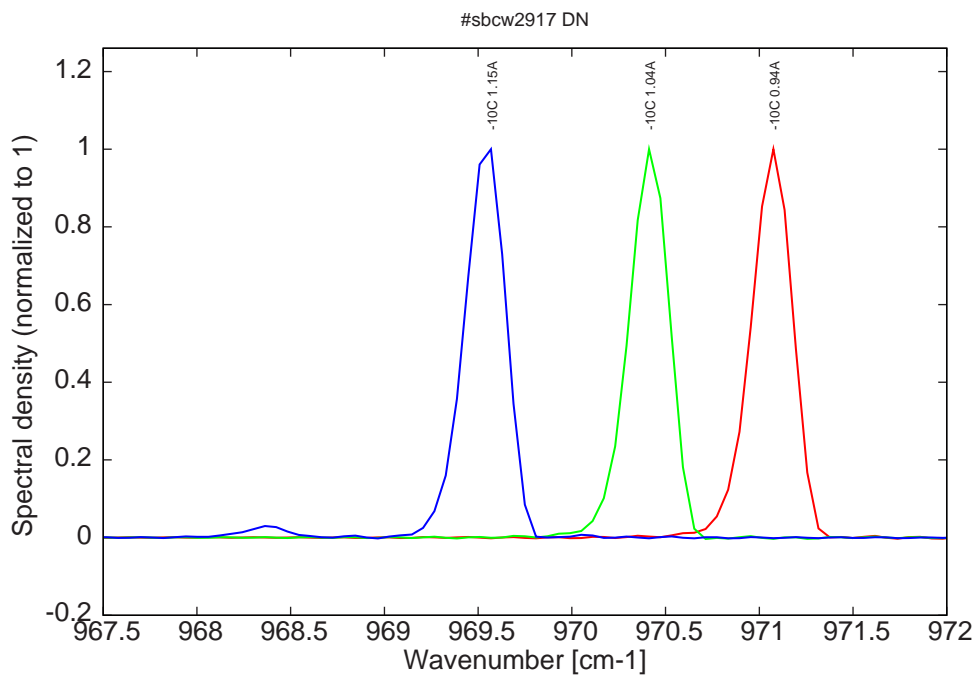
Figure 7: spectra at -10C for various DC currents, monomode up to 1.04A, then bimode
