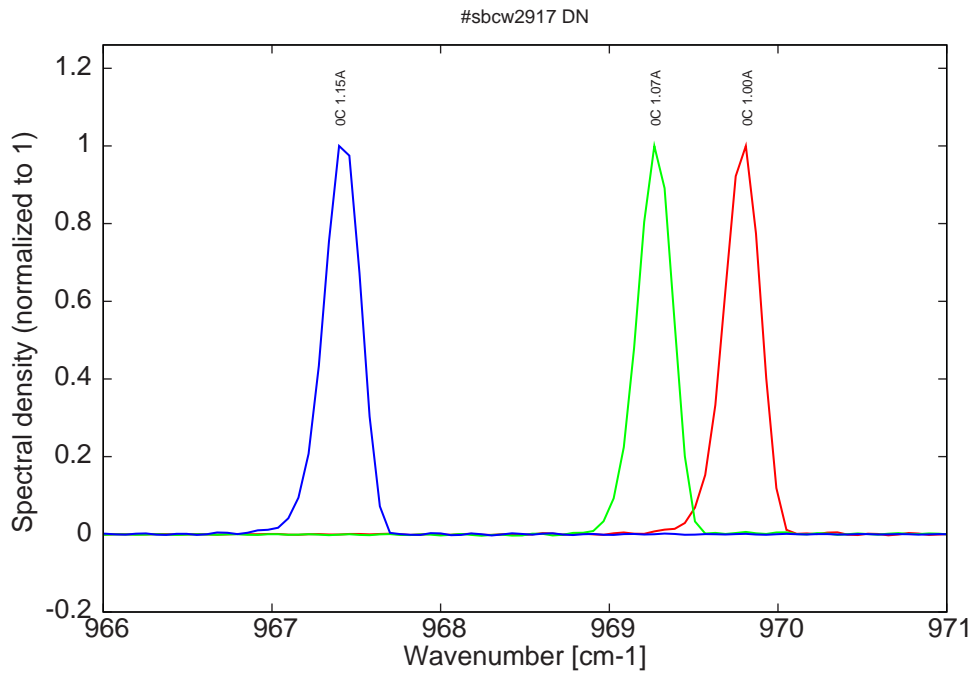
Figure 8: spectra at 0C for various DC currents, all monomode but with mode jumping for I > 1.07\text{A} (see Fig. 3)
