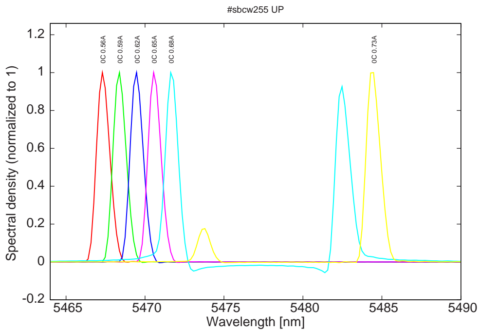
Figure 13: spectra at 0C for various DC currents
