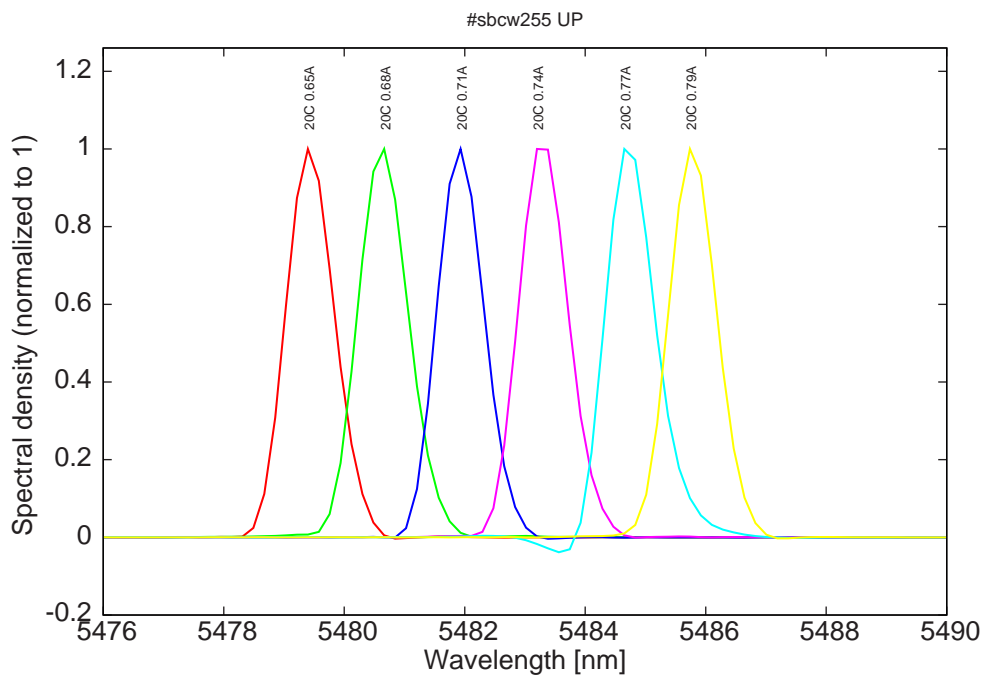
Figure 17: spectra at 20C for various DC currents (monomode)
