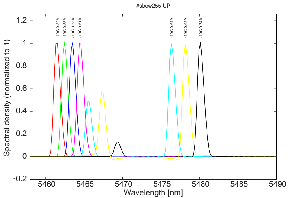
Figure 11: spectra at -10C for various DC currents
