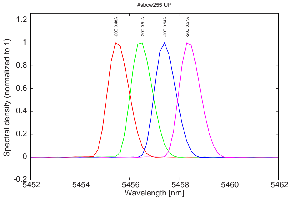
Figure 10: spectra at -20C for various DC currents (monomode range)
