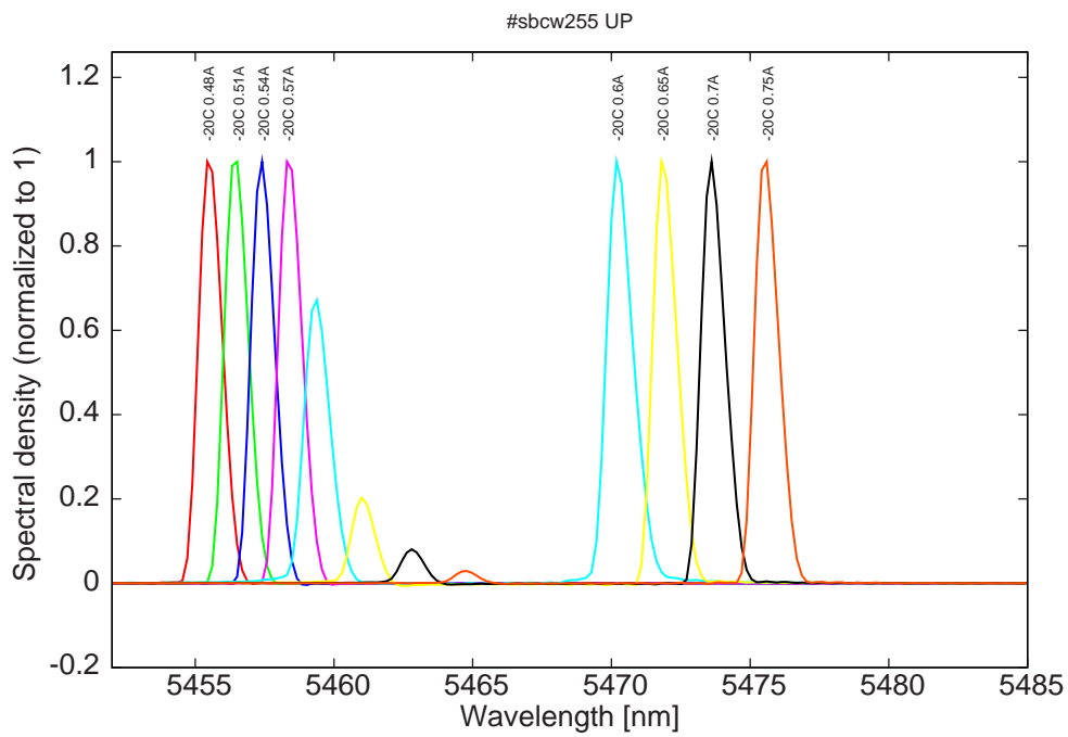
Figure 9: spectra at -20C for various DC currents
