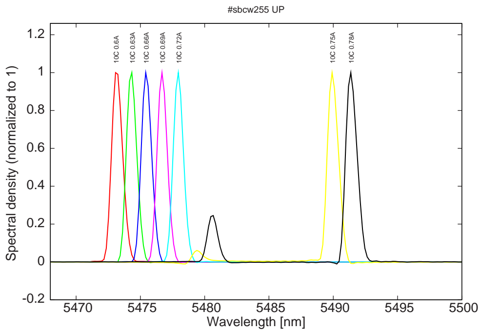
Figure 15: spectra at 10C for various DC currents
