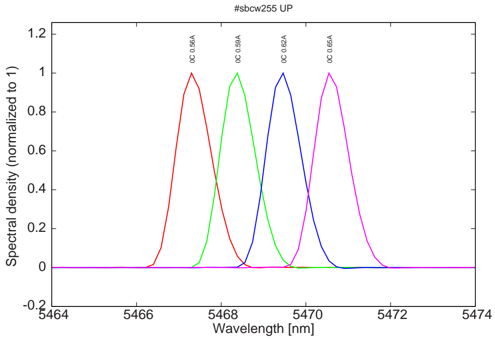
Figure 14: spectra at 0C for various DC currents (monomode range)
