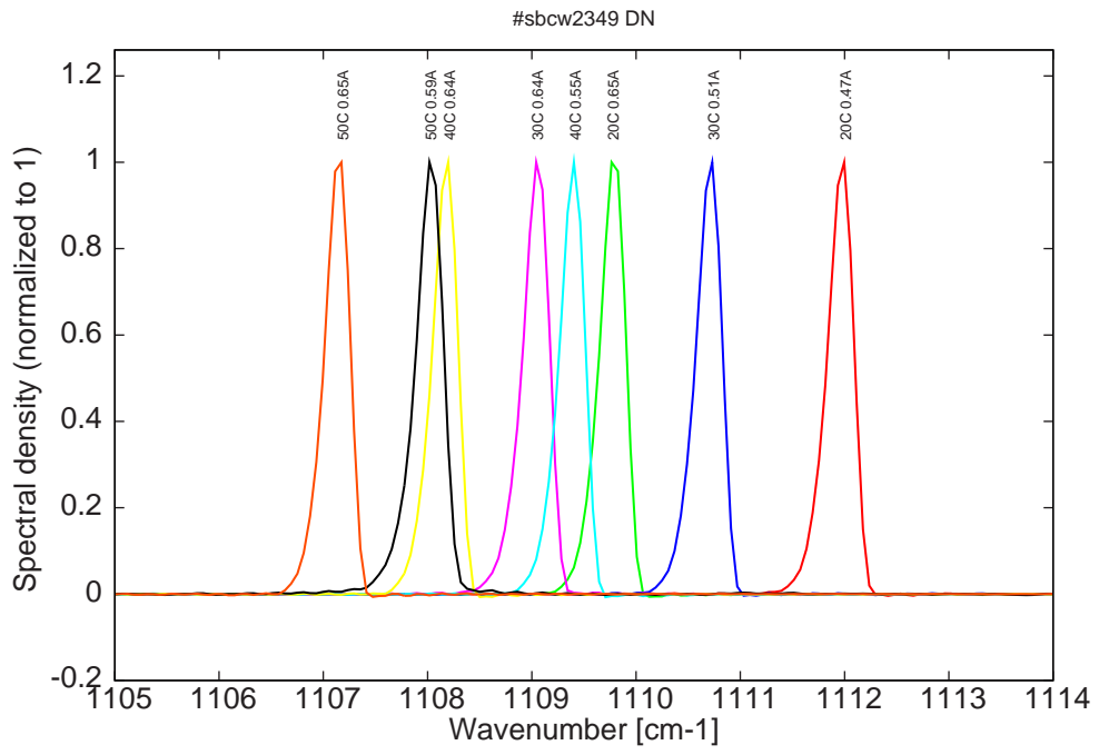
Figure 16: spectra between 20C and 50C for various DC currents (all monomode)
