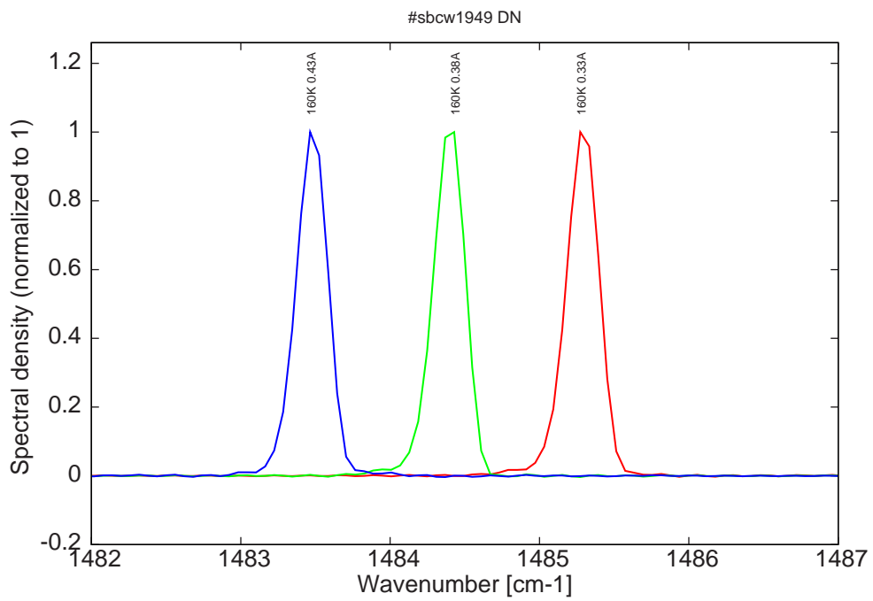
Figure 15: spectra at 160K for various DC currents (monomode range)
