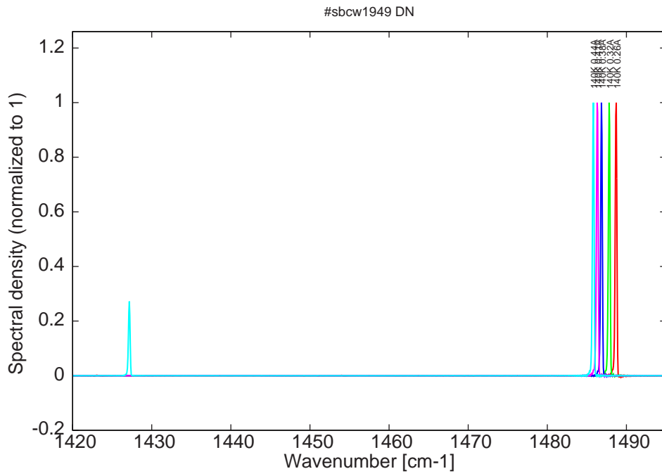
Figure 12: spectra at 140K for various DC currents
