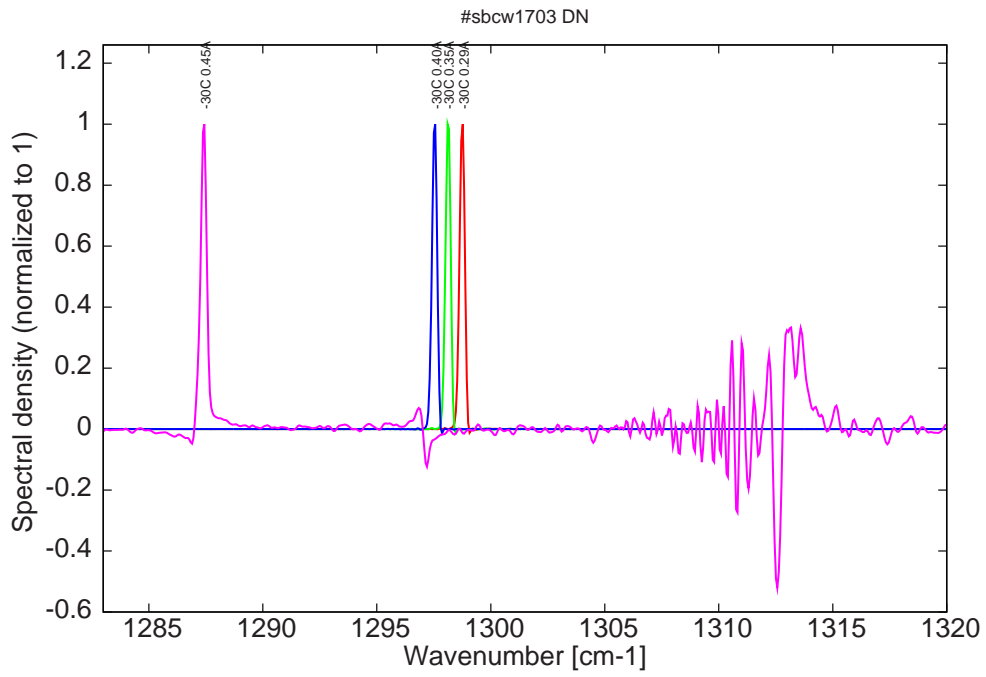
Figure 6: spectra at -30C for various DC currents (monomode up to 0.40A)
