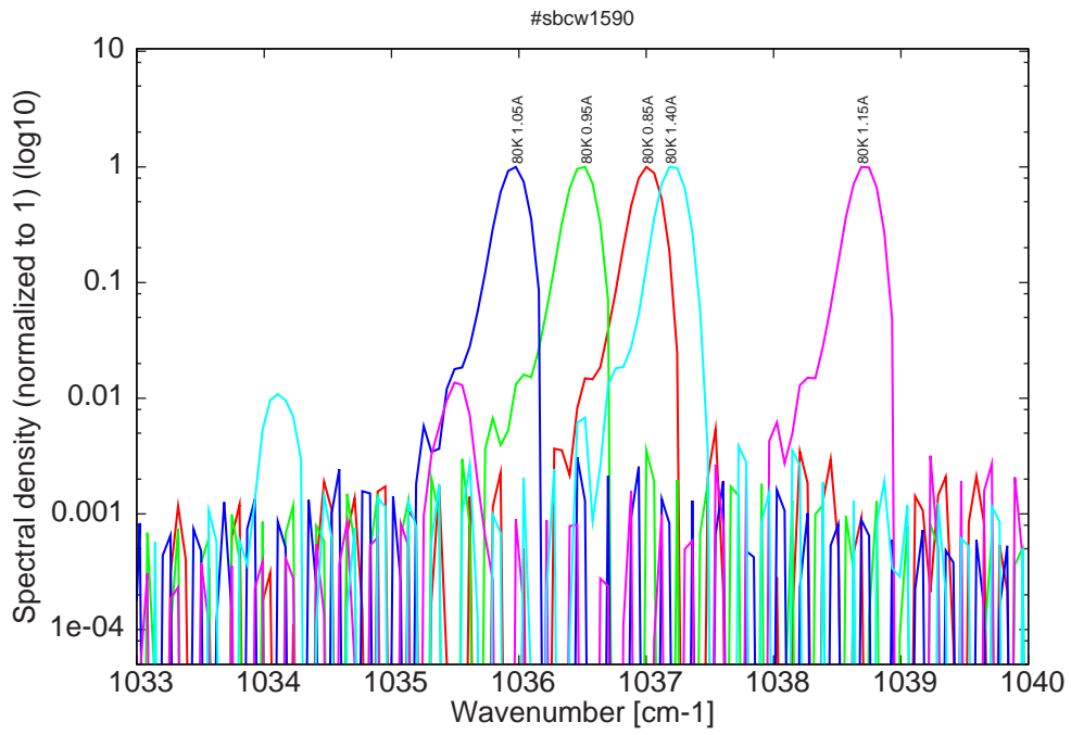
Figure 6: spectra at 80K for various DC currents (mode jumping + bimode for I > 1.05A )
