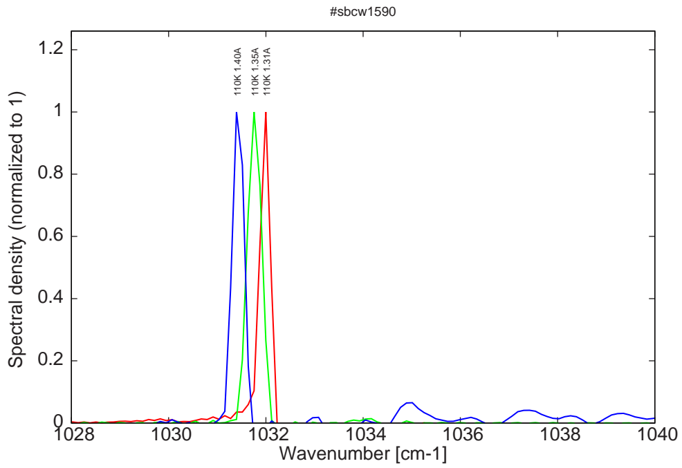
Figure 10: spectra at 110K for various DC currents
