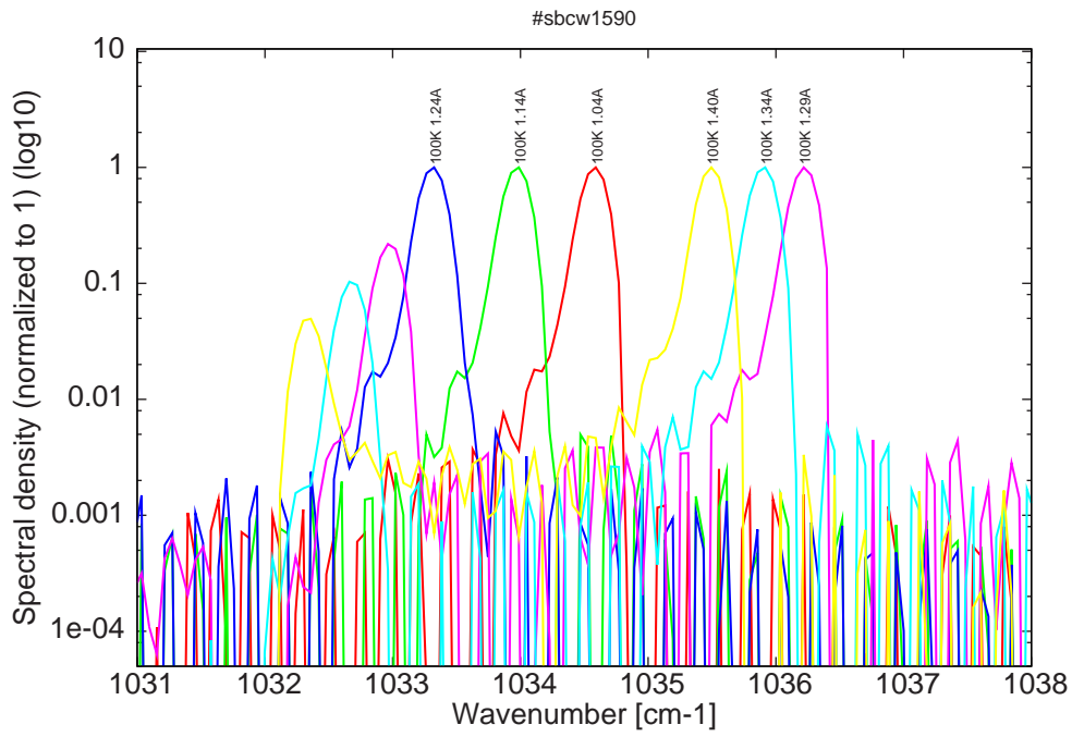
Figure 8: spectra at 100K for various DC currents (bimode for I > 1.24A )
