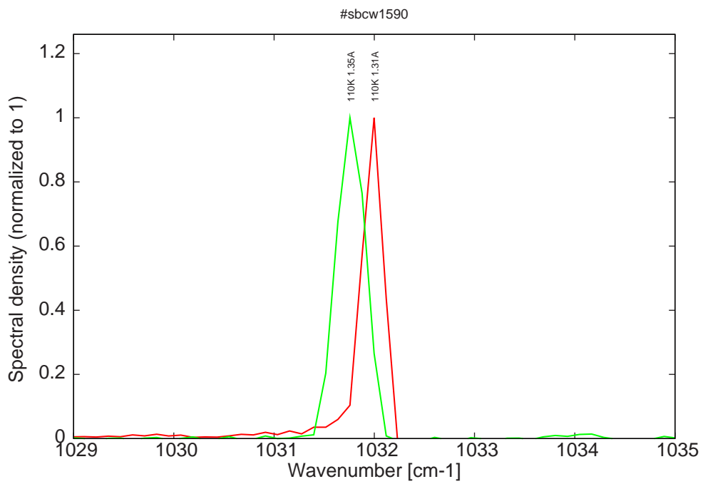
Figure 11: spectra at 110K for various DC currents (monomode range)
