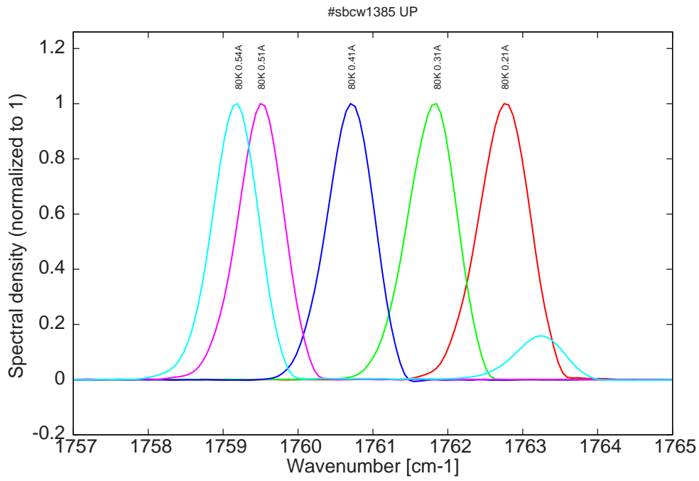
Figure 6: spectra at 80K for various DC currents (monomode up to 0.51A)
