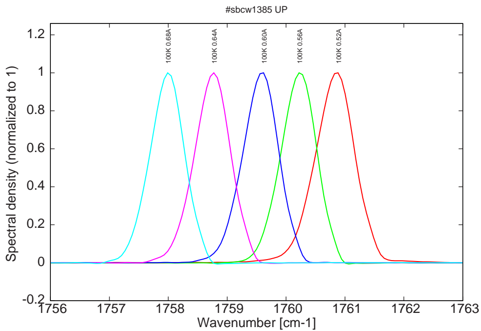
Figure 7: spectra at 100K for various DC currents (all monomode, but not on the same mode as at 80K, see Fig. 1)
