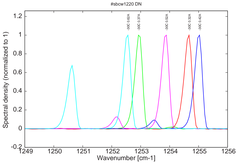
Figure 6: spectra at -30C for various DC currents (monomode at I_{th} but jumping mode compared to other temperatures)
