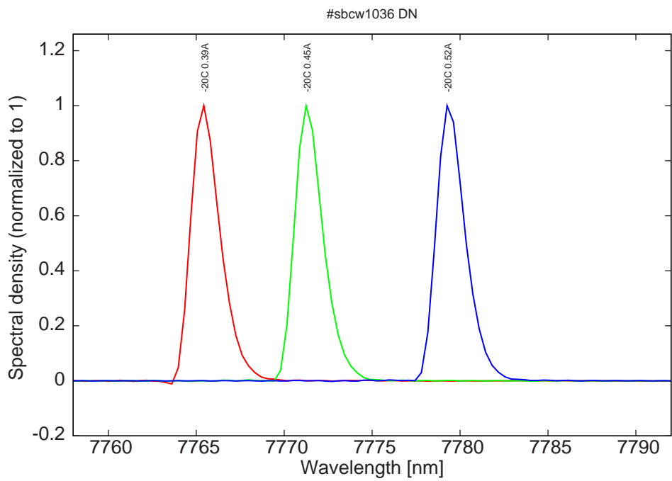
Figure 6: spectra at -20C for various DC currents
