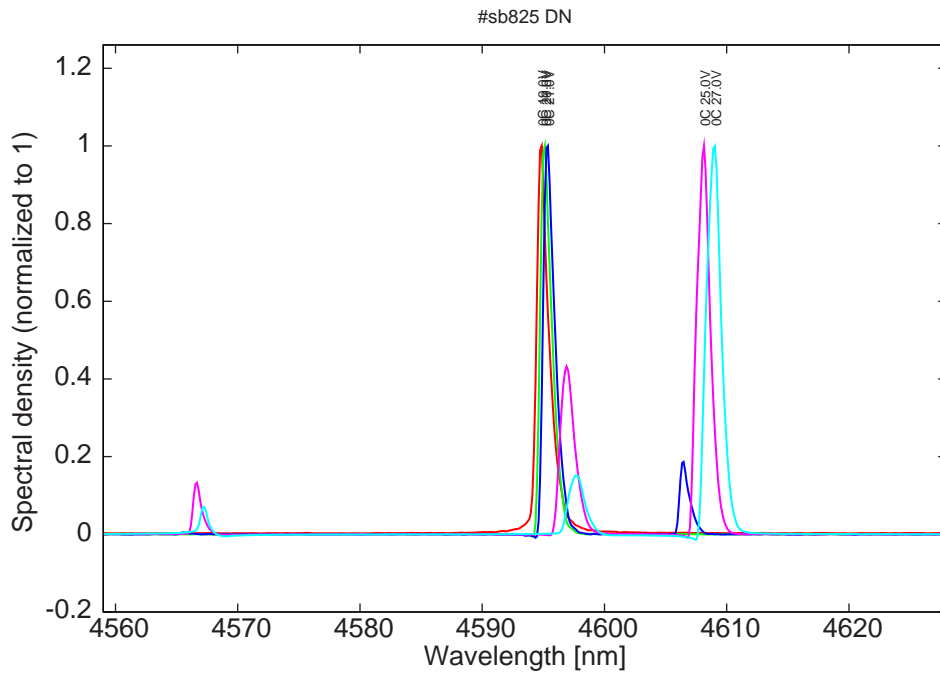
Figure 13: spectra at 0C for various LDD voltages (monomode up to 20V)
