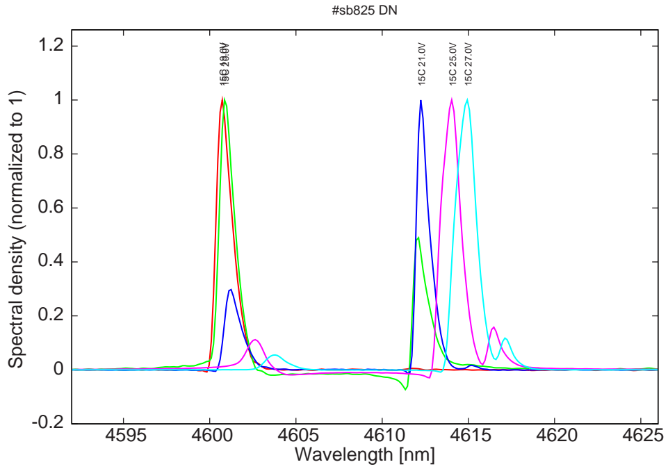
Figure 15: spectra at 15C for various LDD voltages (monomode just at threshold)
