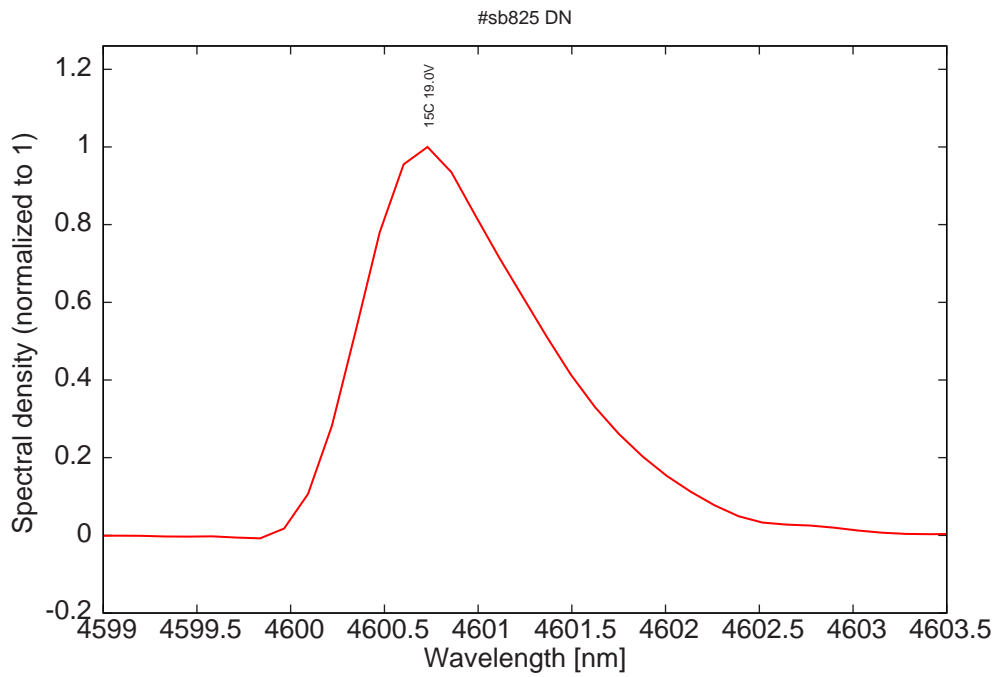
Figure 16: monomode spectrum at 15C and 19V
