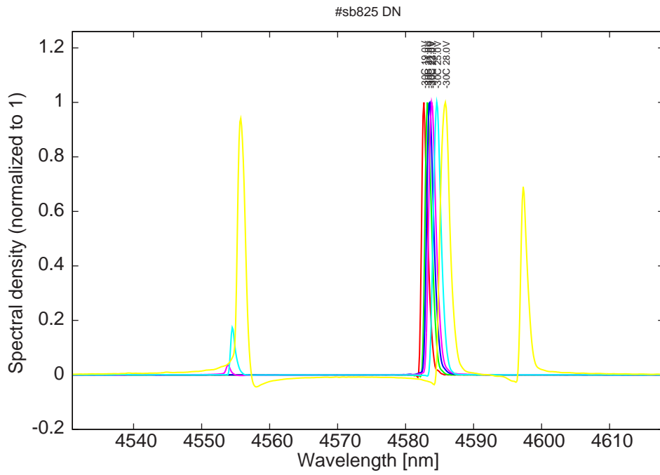
Figure 9: spectra at -30C for various LDD voltages (monomode up to 22V)
