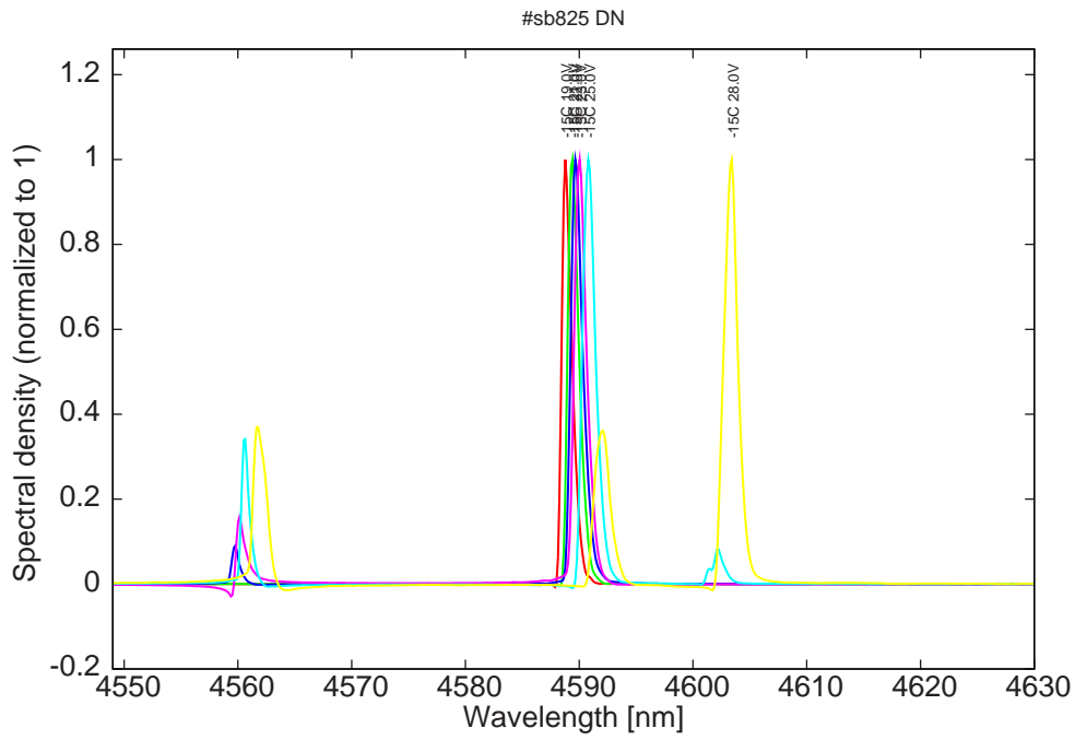
Figure 11: spectra at -15C for various LDD voltages (monomode up to 21V)
