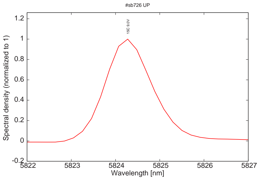
Figure 10: spectrum at 15C and 9.0V on LDD (too much absorption in the air for voltages < 9.0V)
