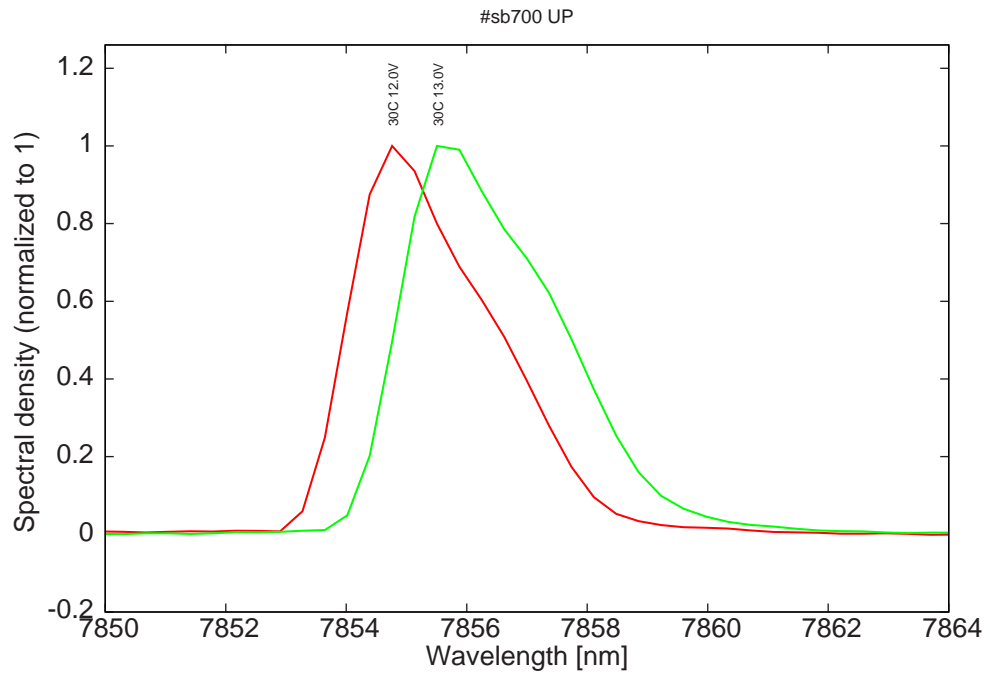
Figure 11: spectra at 30C for various LDD voltages
