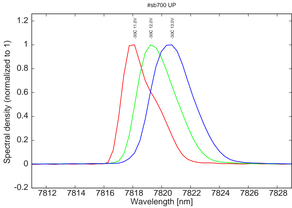
Figure 7: spectra at -30C for various LDD voltages
