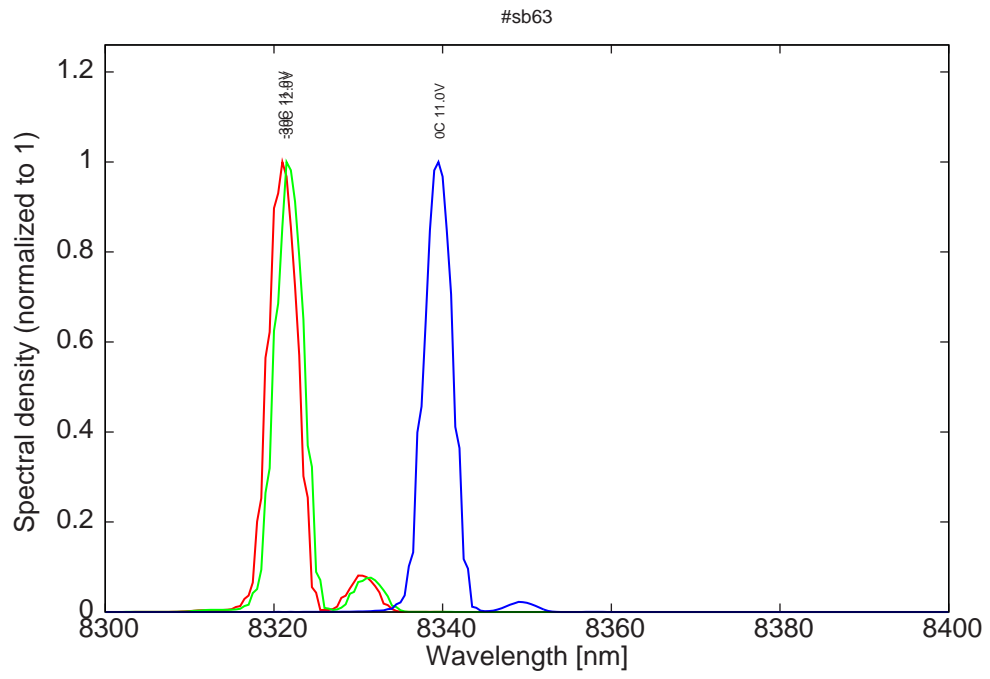
Figure 9: bimode spectra for low temperatures and LDD voltages
