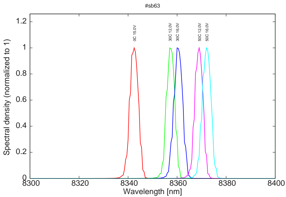
Figure 8: monomode spectra for higher temperatures and LDD voltages
