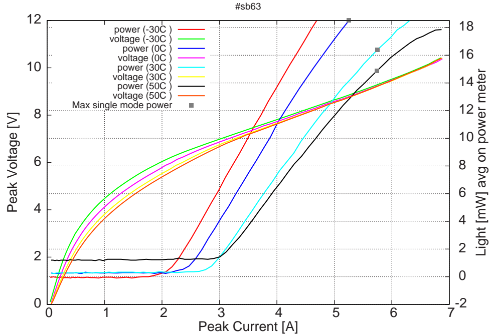
Figure 4: peak voltage and avg power vs peak current (the solid squares indicate the maximum singlemode emitted power)
