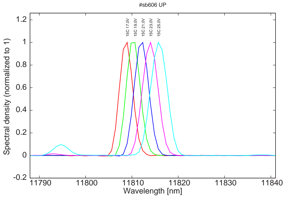
Figure 15: spectra at 15C for various LDD voltages
