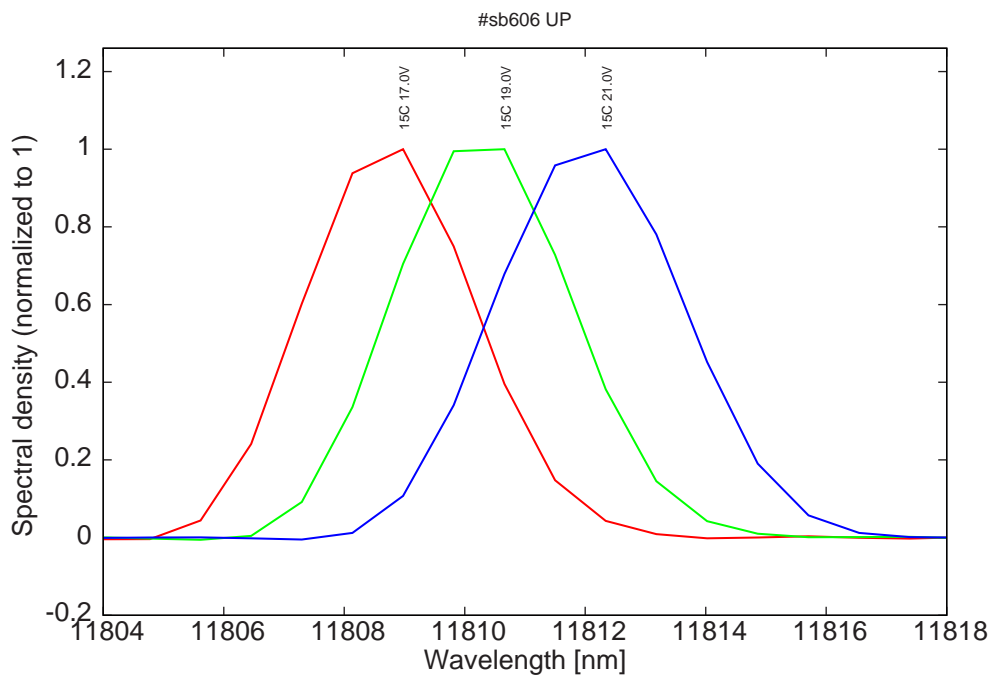
Figure 16: spectra at 15C for various LDD voltages (monomode range)
