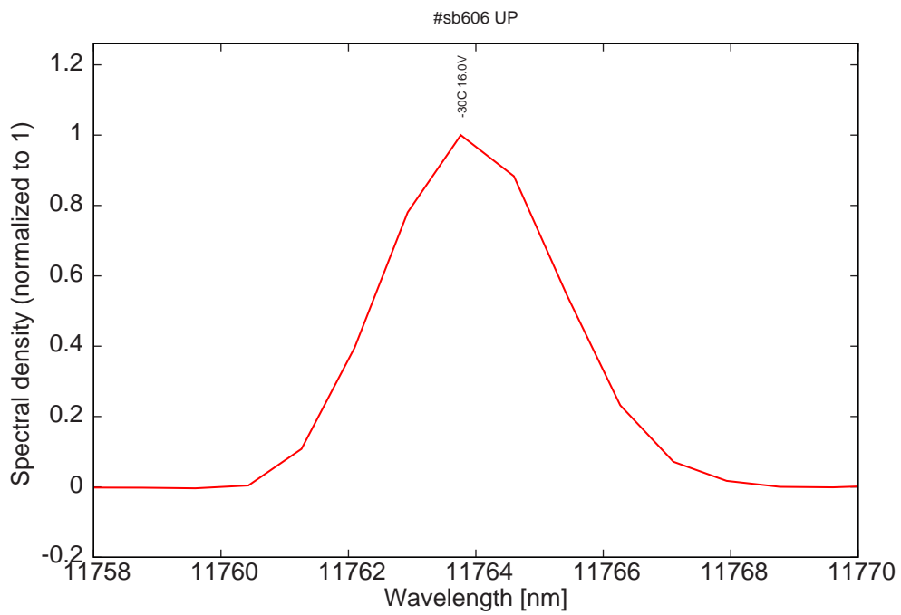
Figure 10: monomode spectrum at -30C at 16.0V on LDD
