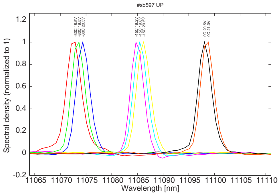
Figure 6: spectra at -30C, -15C and 0C at 2% dc for various LDD voltages
