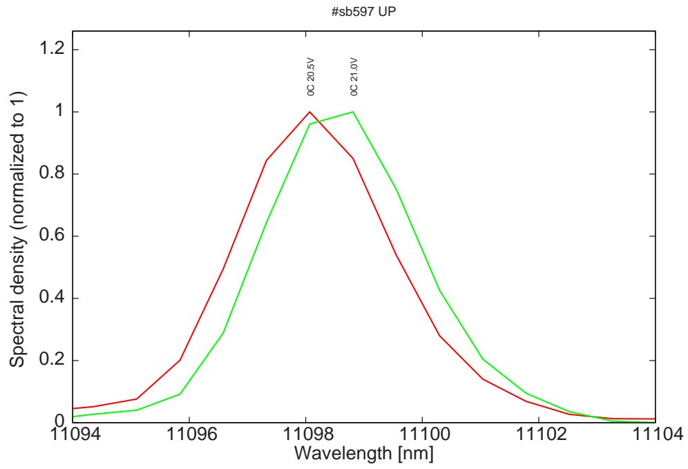
Figure 9: spectra at 0C for various LDD voltages
