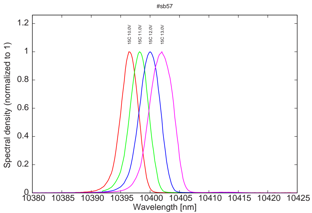
Figure 12: spectra at 15C for various LDD voltages (bimode at 13V)
