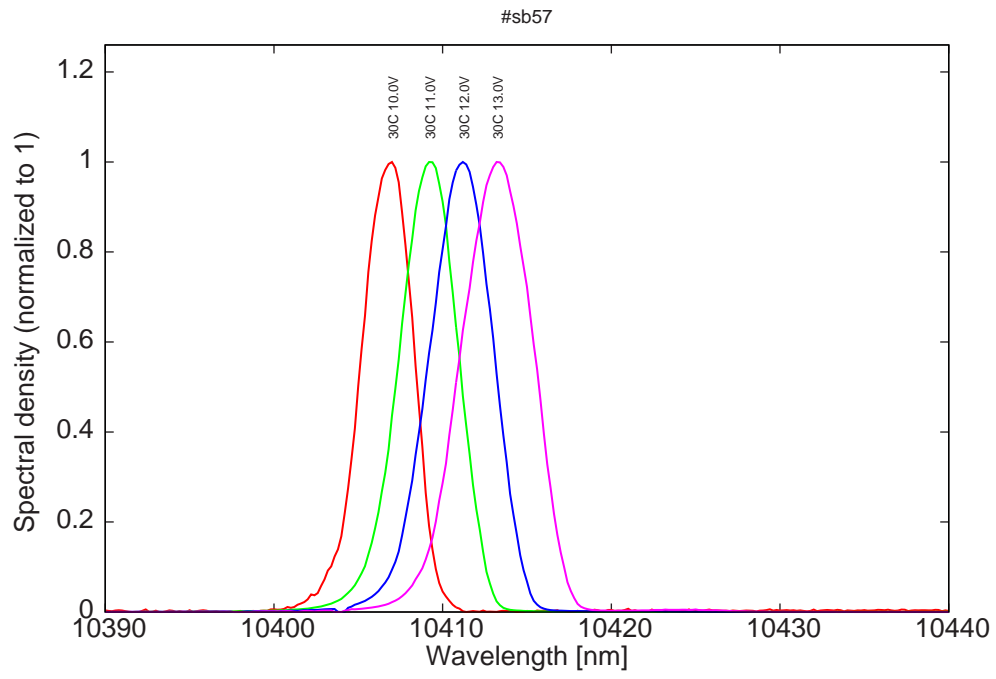
Figure 13: spectra at 30C for various LDD voltages (bimode at 13V)
