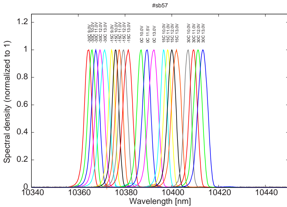
Figure 8: spectra for various temperatures and LDD voltages
