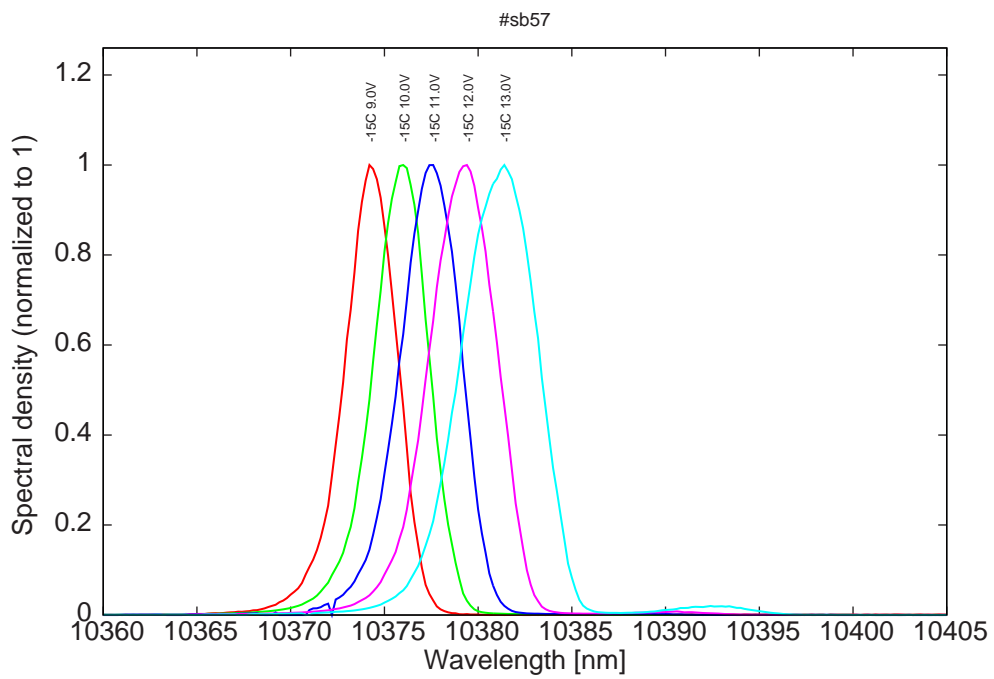
Figure 10: spectra at -15C for various LDD voltages (bimode at 12 and 13V)
