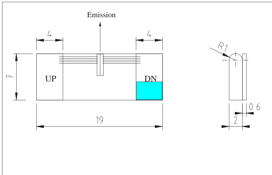
Figure 1: Support mounting for #sb57 (please note that the laser is connected to the DN pad drawn in blue)
