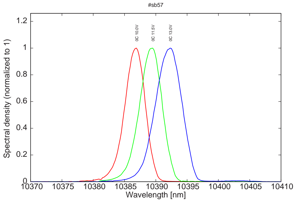
Figure 11: spectra at 0C for various LDD voltages (bimode at 13V)
