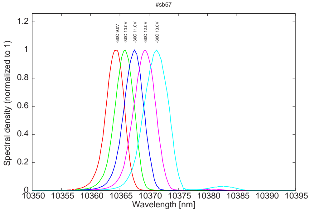
Figure 9: spectra at -30C for various LDD voltages (bimode at 12 and 13V)
