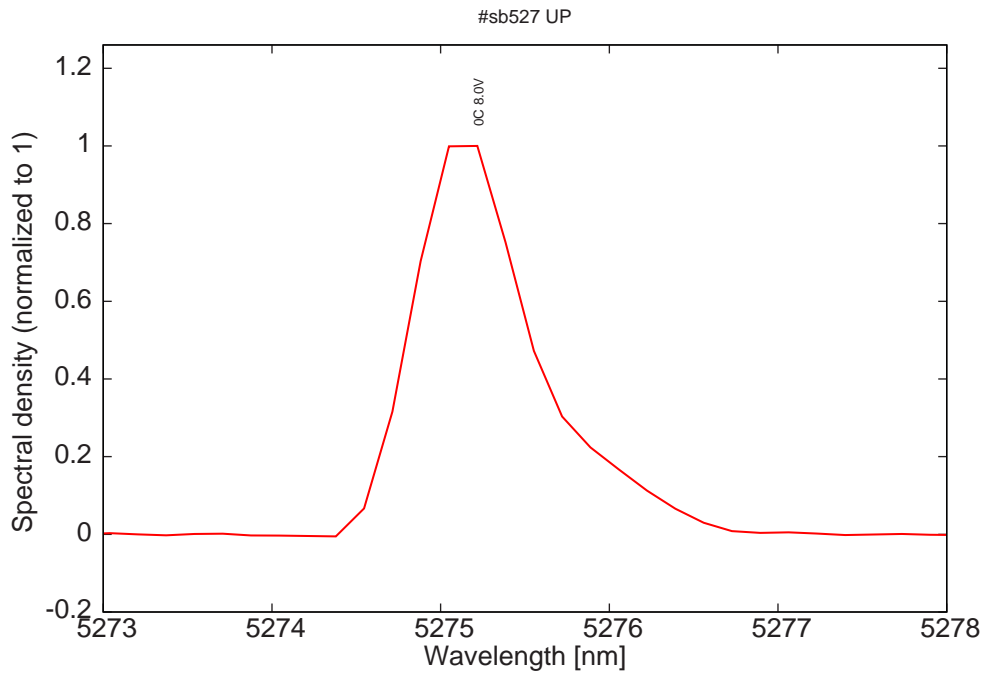
Figure 11: monomode spectrum at 0C and 8V on LDD
