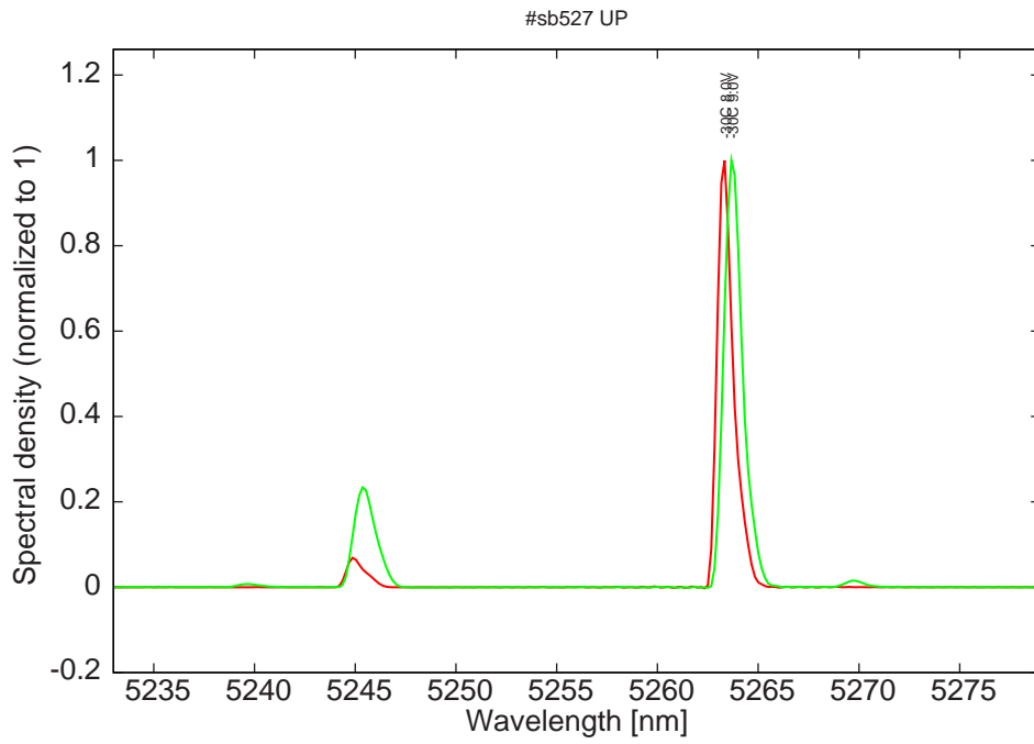
Figure 9: spectra at -30C for various LDD voltages (multimode)
