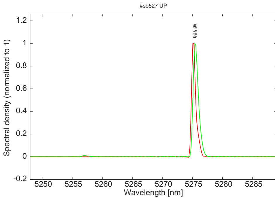
Figure 10: spectra at 0C for various LDD voltages
