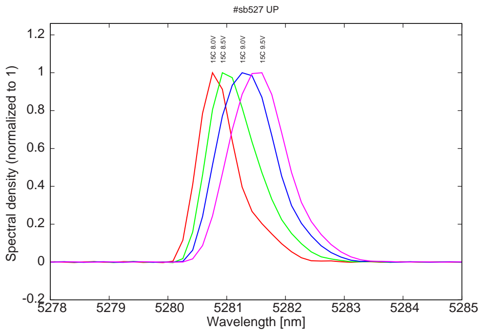
Figure 12: spectra at 15C for various LDD voltages (become bimode > 9.5V)
