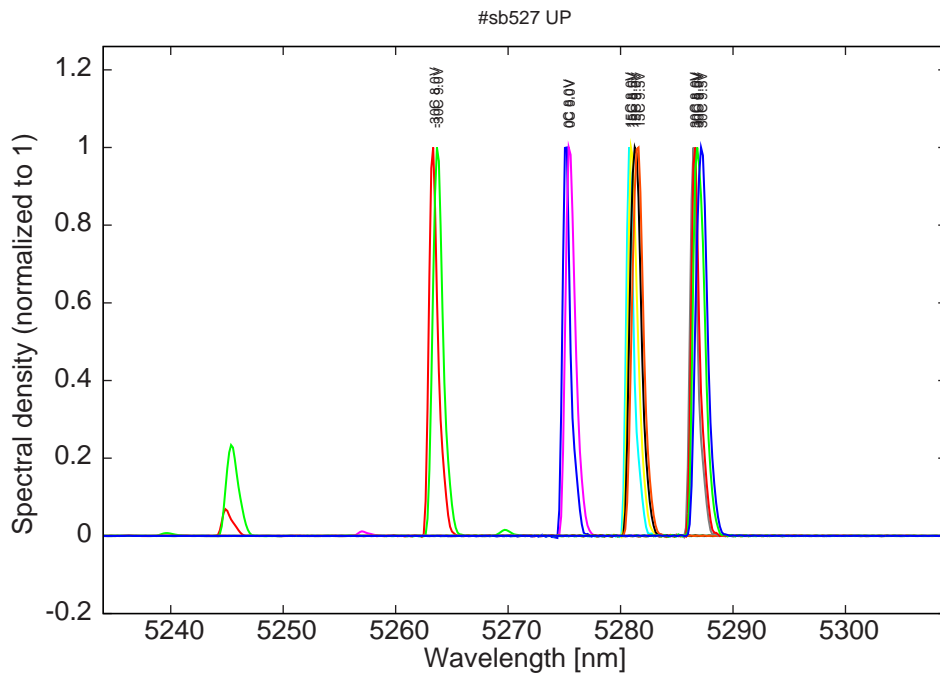
Figure 8: spectra at -30C, 0C, 15C and 30C at 2% dc for various LDD voltages
