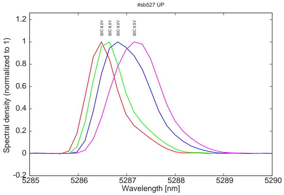
Figure 13: spectra at 30C for various LDD voltages
