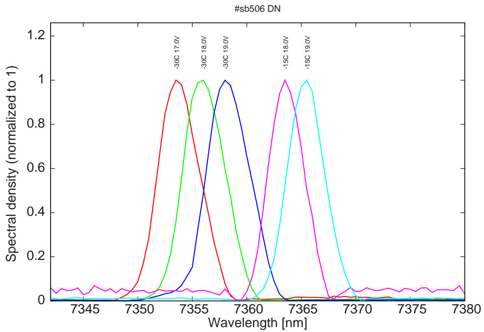
Figure 6: spectra at -30C and -15C at 2% dc for various LDD voltages
