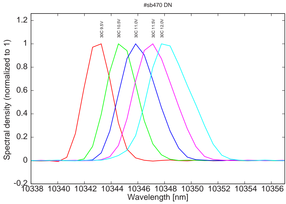
Figure 11: spectra at 30C for various LDD voltages
