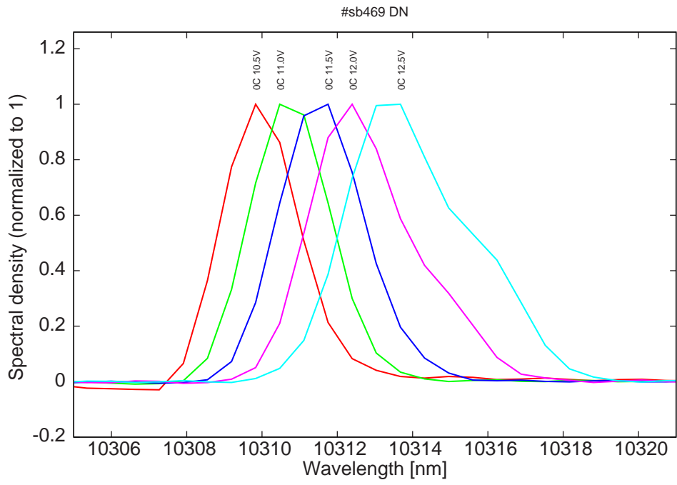
Figure 13: spectra at 0C for various LDD voltages (all monomode)
