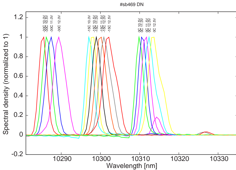
Figure 8: spectra at -30C, -15C and 0C 2% dc for various LDD voltages
