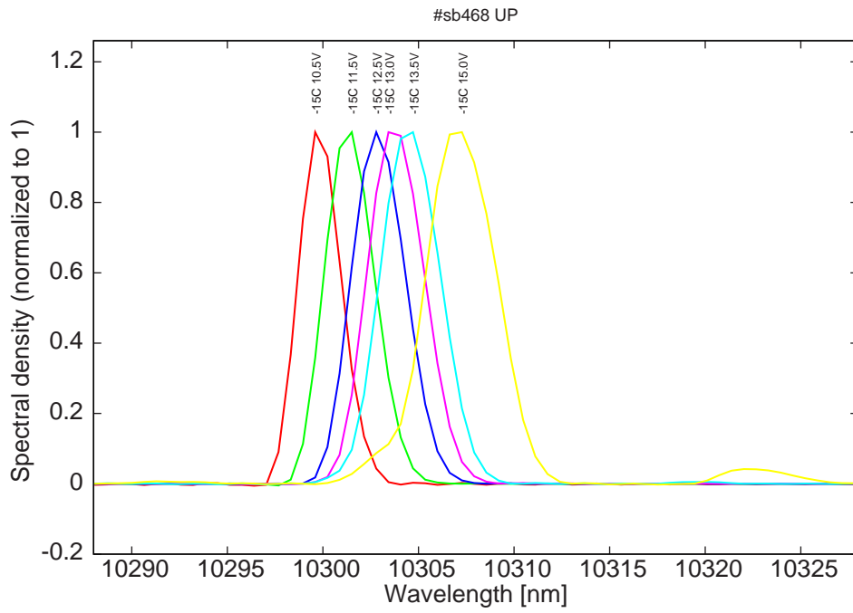
Figure 11: spectra at -15C for various LDD voltages
