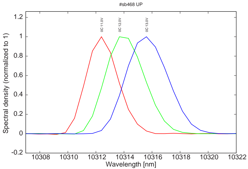
Figure 14: spectra at 0C for various LDD voltages (monomode range)
