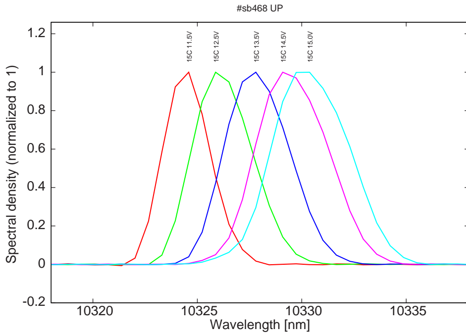
Figure 15: spectra at 15C for various LDD voltages (all monomode)
