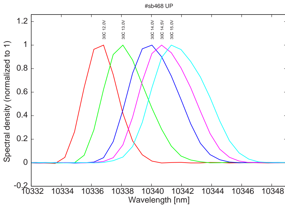
Figure 16: spectra at 30C for various LDD voltages (all monomode)
