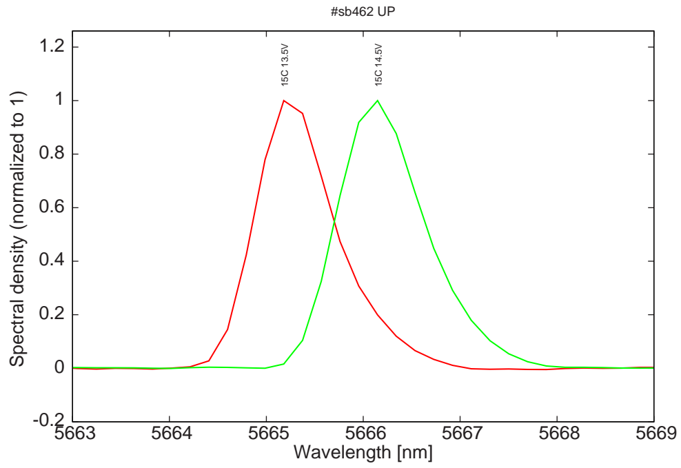
Figure 15: spectra at 15C for various LDD voltages (monomode)
