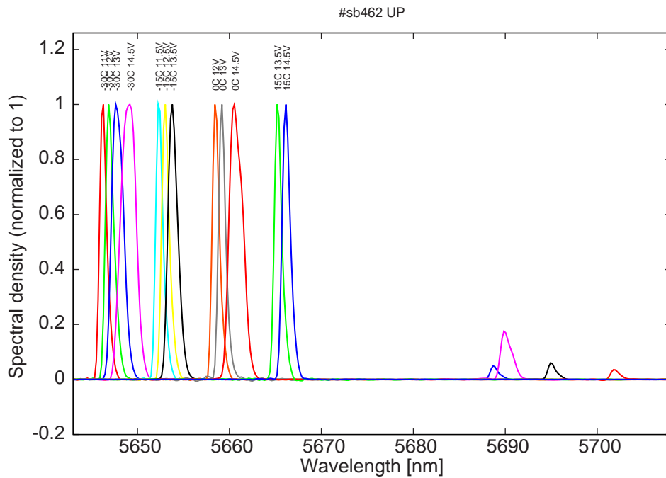
Figure 8: spectra at -30C, -15C, 0C and 15C at 4% dc for various LDD voltages
