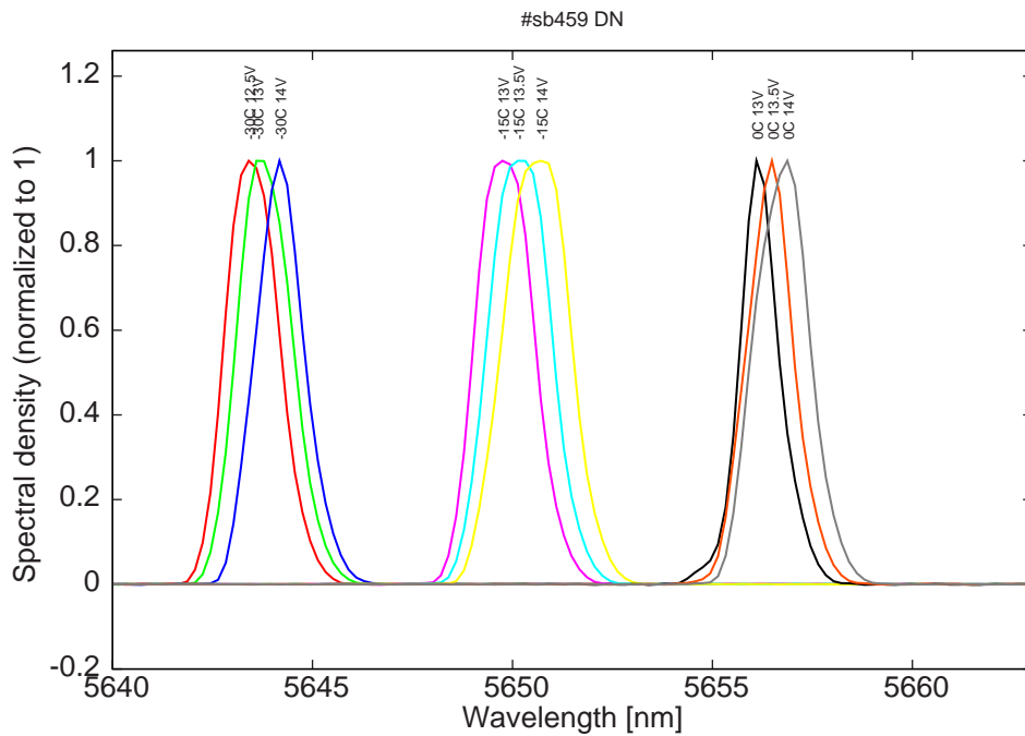
Figure 6: spectra at -30C, -15C and 0C at 4% dc for various LDD voltages
