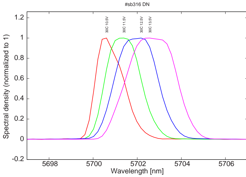
Figure 15: spectra at 30C for various LDD voltage
