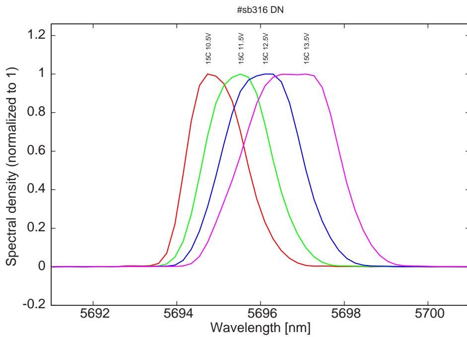
Figure 14: spectra at 15C for various LDD voltage
