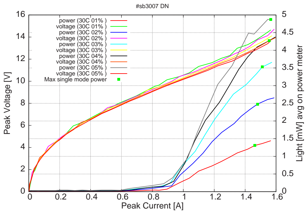
Figure 17: peak voltage and average power vs peak current at 30C for various duty-cycles (100ns pulses on the laser)
