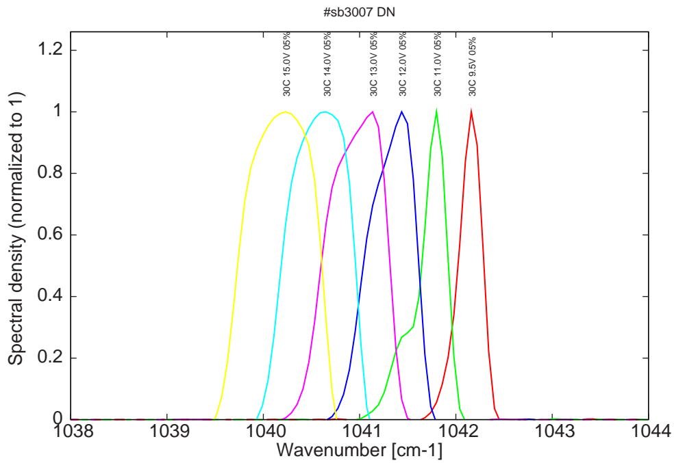
Figure 19: spectra at 30C at 5% duty-cycle for various LDD voltages (all monomode)
