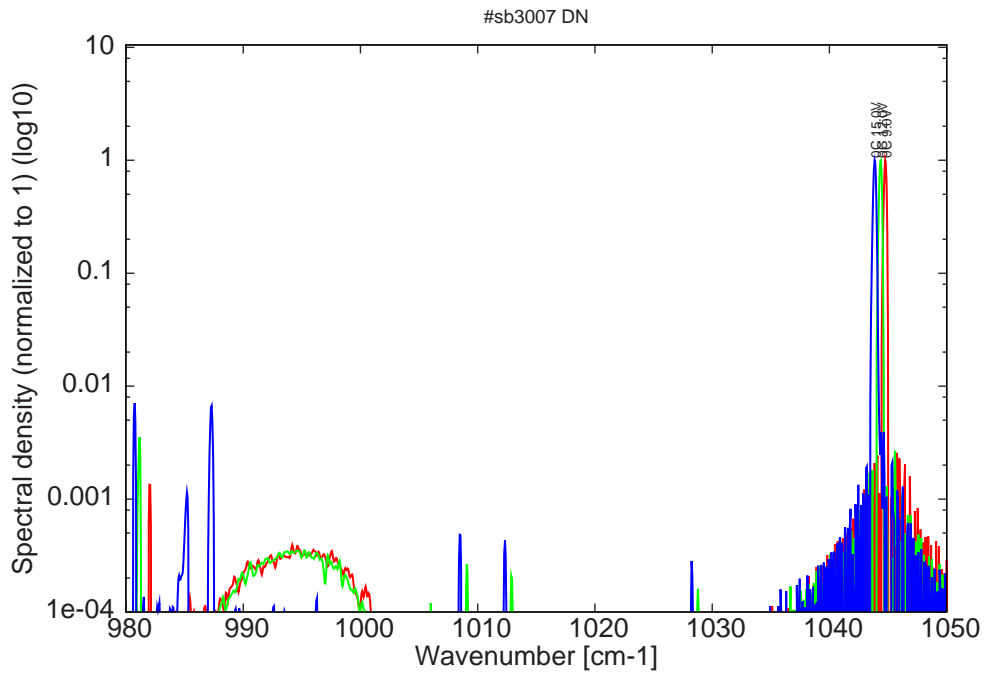
Figure 12: spectra at 0C for various LDD voltages (monomode up to 12V on LDD)
