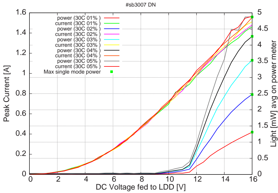
Figure 18: peak current and average power vs LDD voltage at 30C for various duty-cycles (100ns pulses on the laser)
