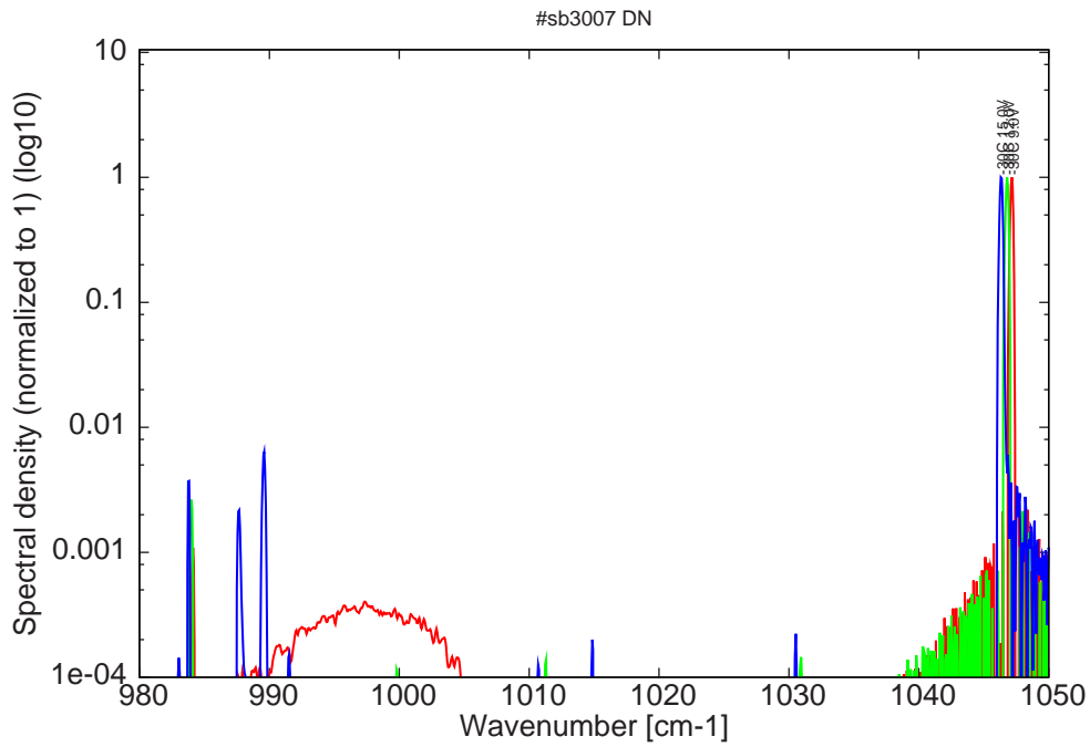
Figure 8: spectra at -30C for various LDD voltages (monomode up to 12V on LDD)
