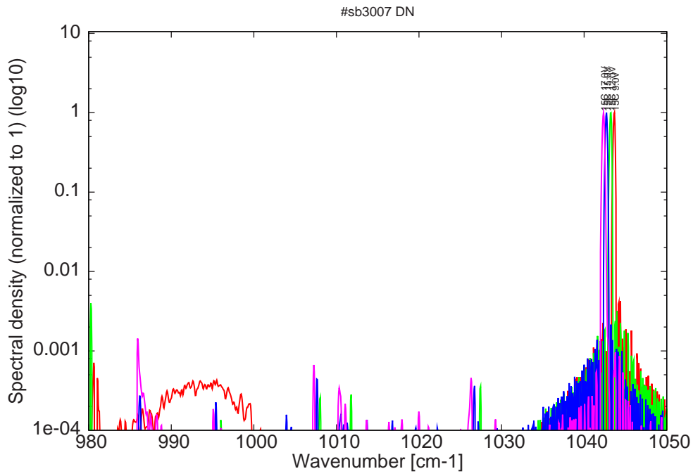
Figure 14: spectra at 15C for various LDD voltages (monomode up to 15V on LDD)
