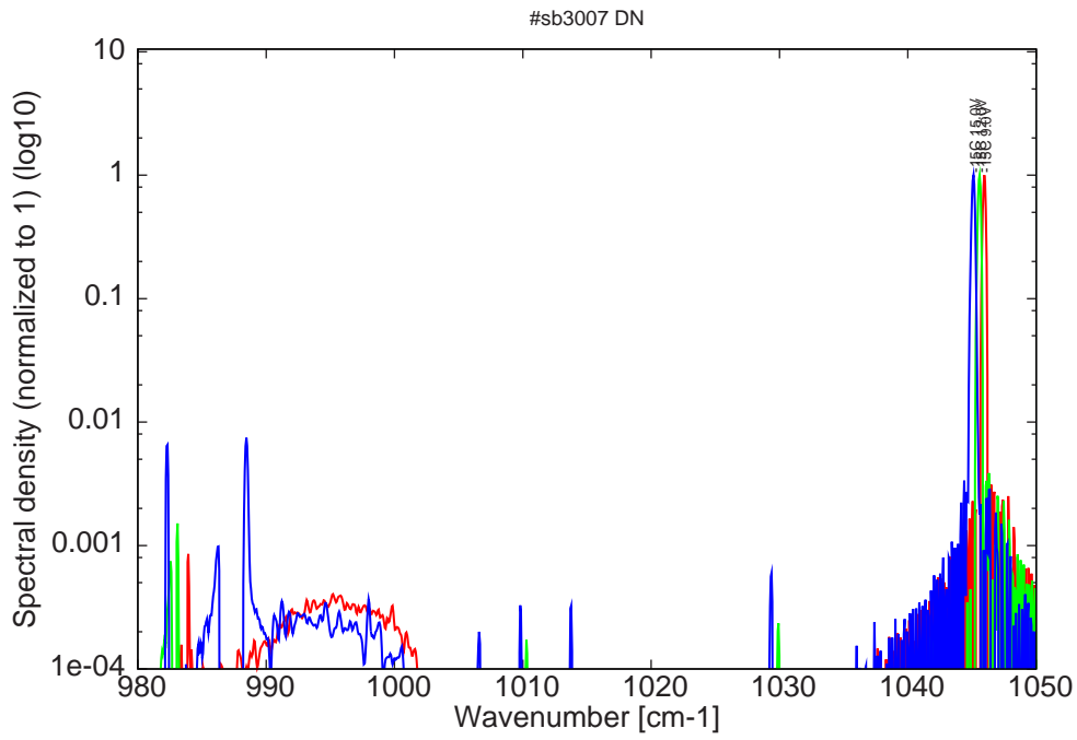
Figure 10: spectra at -15C for various LDD voltages (monomode up to 12V on LDD)
