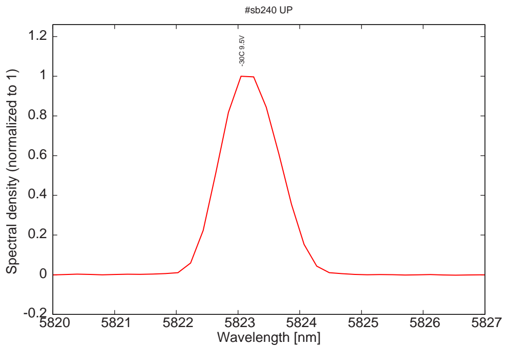
Figure 10: spectrum at -30C and at 9.5V (monomode)
