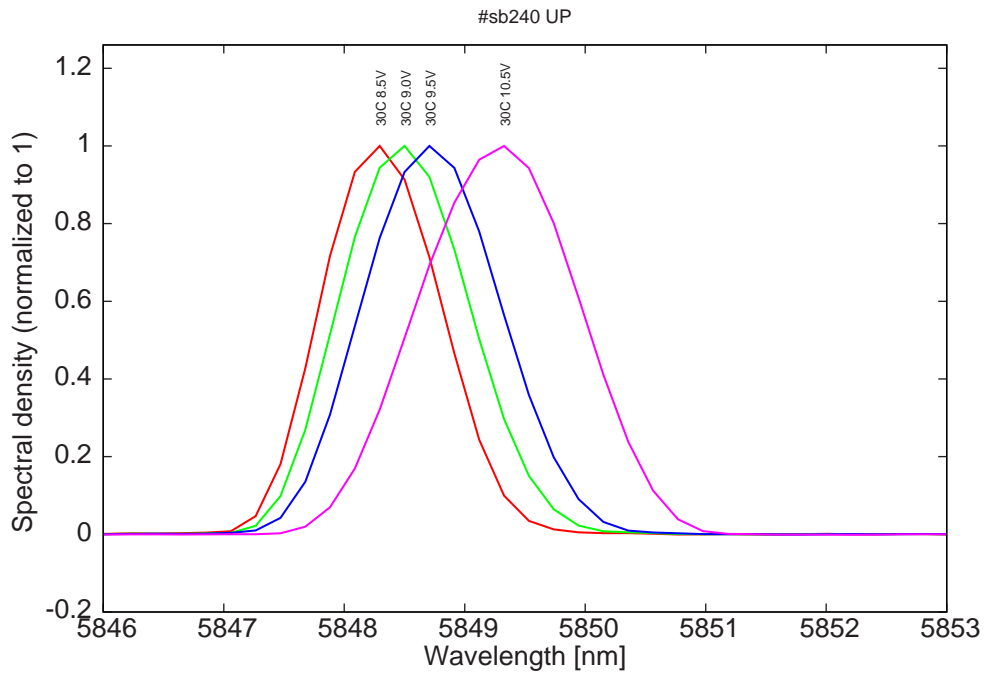
Figure 15: spectra at 30C for various LDD voltage
