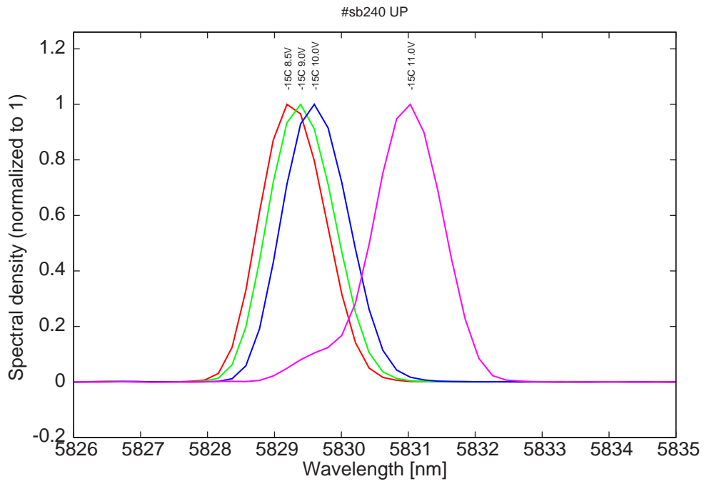
Figure 11: spectra at -15C for various LDD voltage
