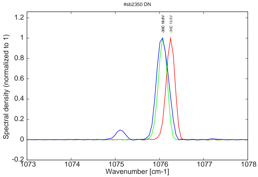
Figure 8: spectra at -30C for various LDD voltages (monomode up to 16.5V)
