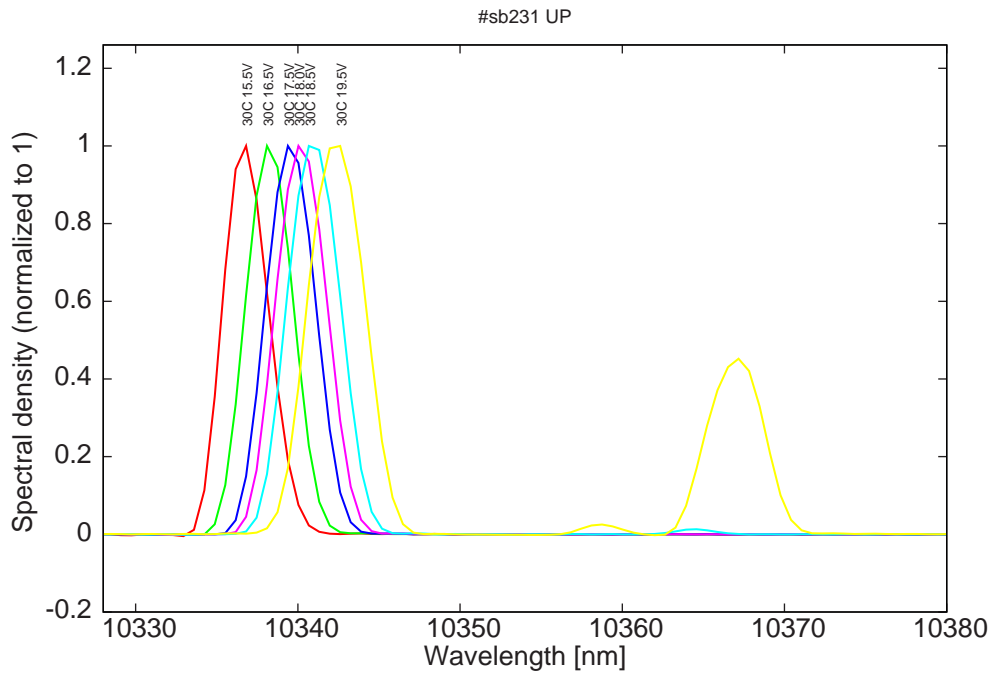
Figure 17: spectra at 30C for various LDD voltages
