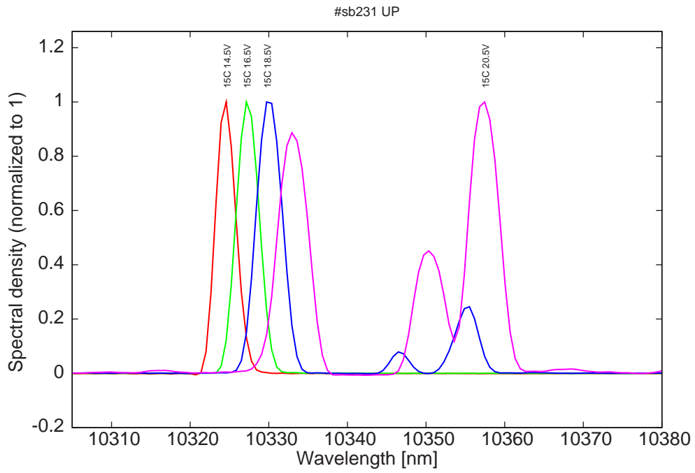
Figure 15: spectra at 15C for various LDD voltages
