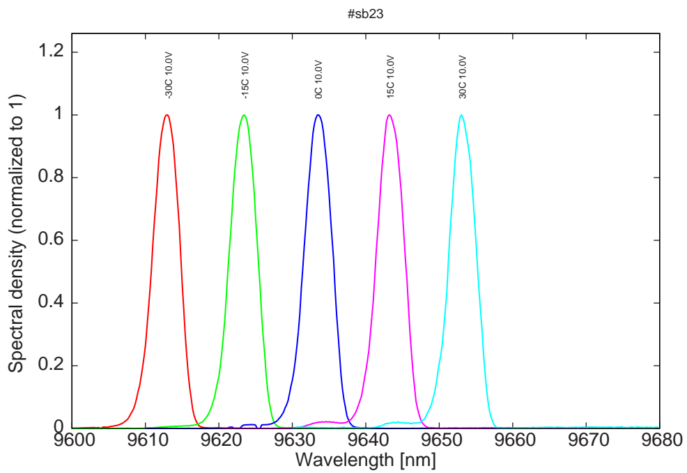
Figure 8: spectra for various temperatures and 10V on LDD
