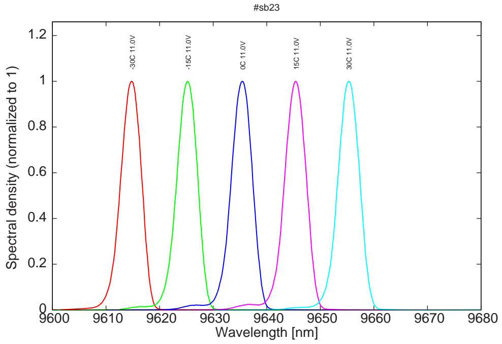
Figure 9: spectra for various temperatures and 11V on LDD
