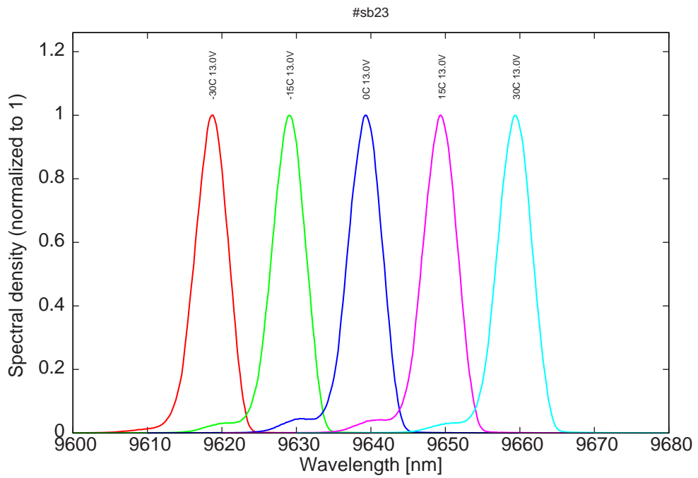
Figure 10: spectra for various temperatures and 13V on LDD
