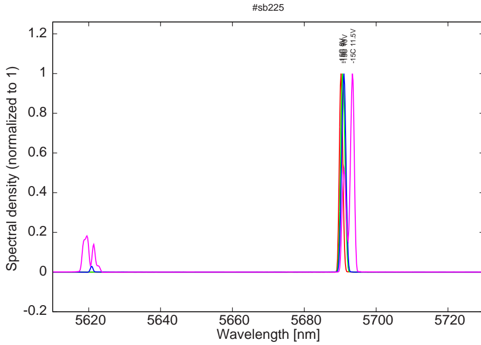
Figure 11: spectra at -15C for various LDD voltage
