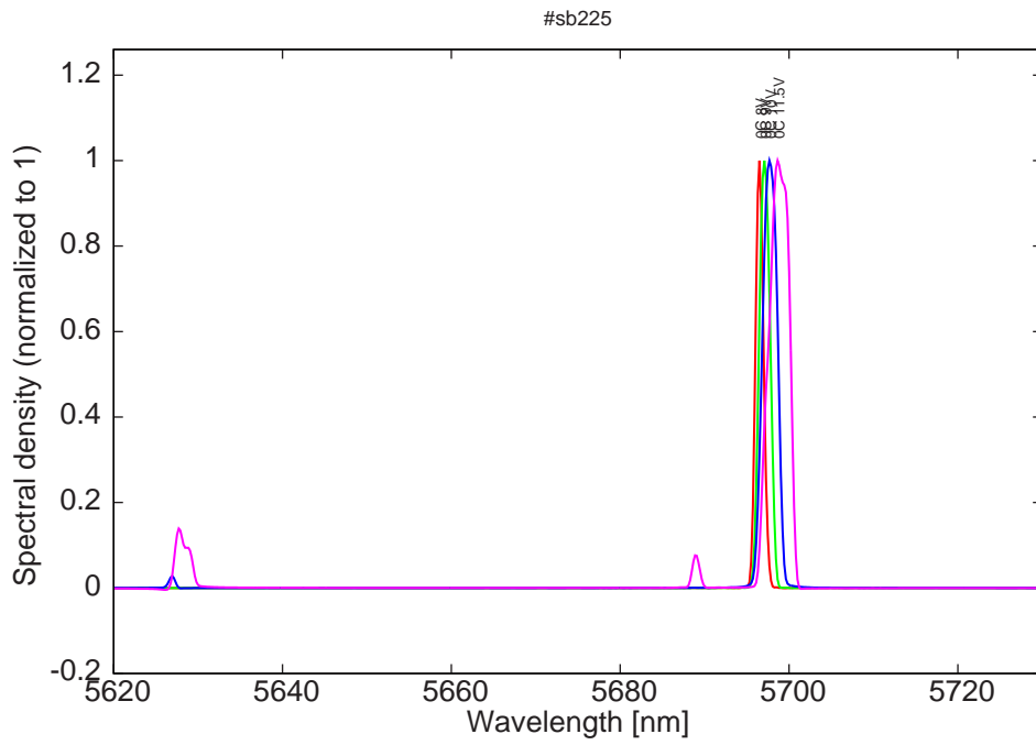
Figure 13: spectra at 0C for various LDD voltage
