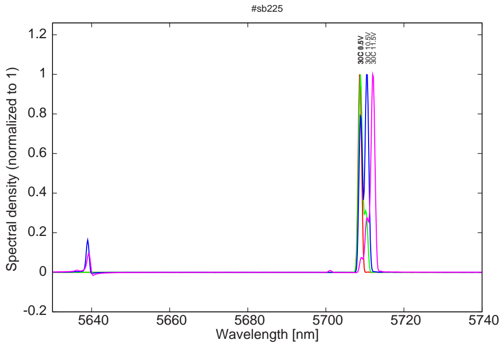
Figure 17: spectra at 30C for various LDD voltage
