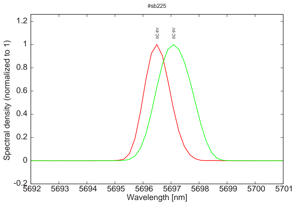
Figure 14: spectra at 0C for various LDD voltage (monomode range)
