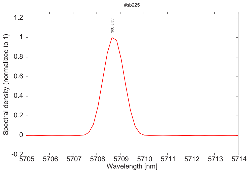
Figure 18: spectrum at 30C and 8.5V (monomode)
