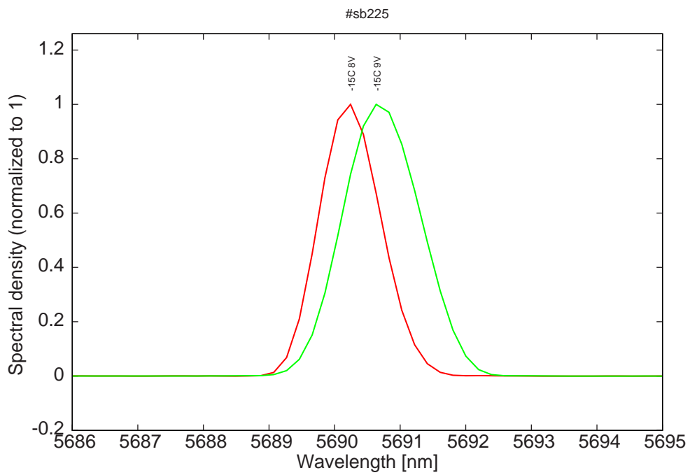
Figure 12: spectra at -15C for various LDD voltage (monomode range)
