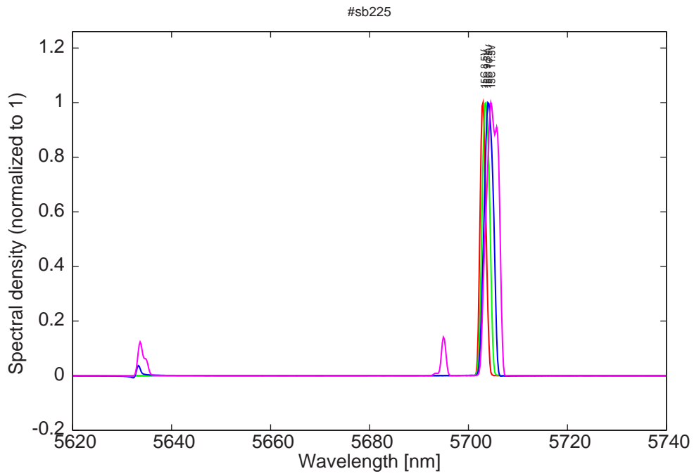
Figure 15: spectra at 15C for various LDD voltage
