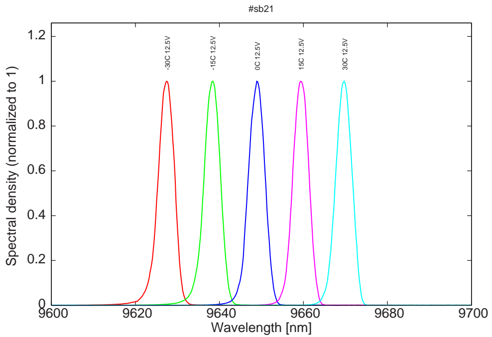
Figure 8: spectra for various temperatures and 12.5V on LDD
