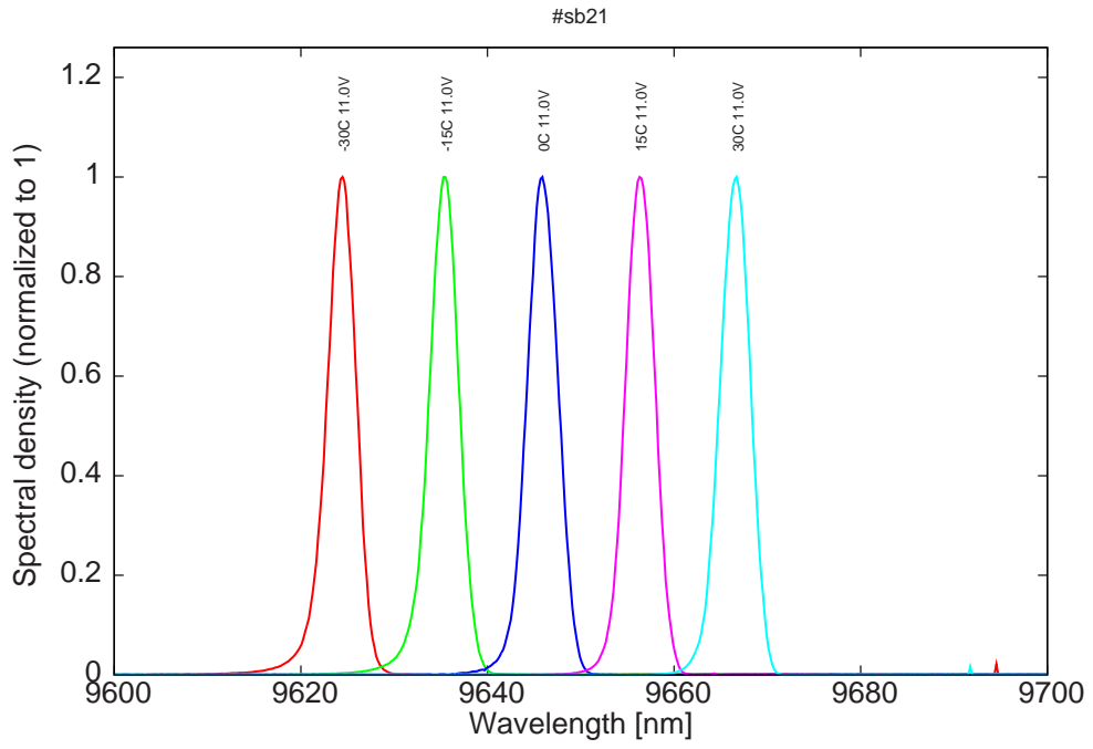
Figure 7: spectra for various temperatures and 11.0V on LDD
