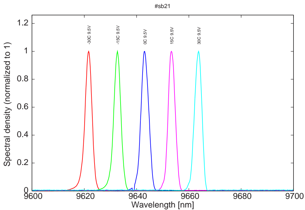
Figure 6: spectra for various temperatures and 9.5V on LDD
