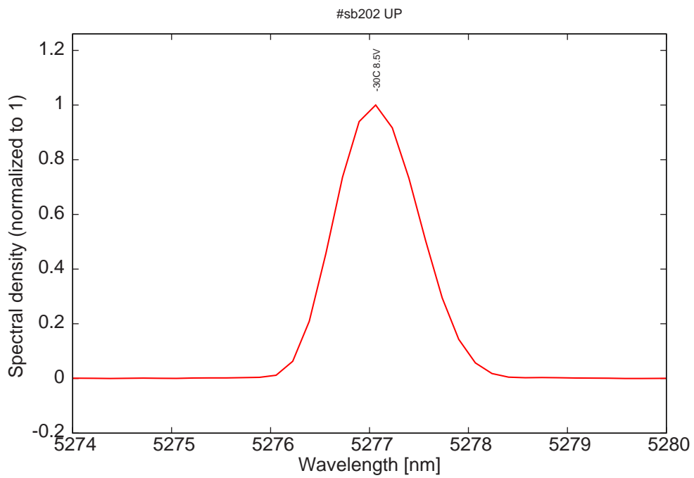
Figure 10: spectrum at -30C and 8.5V on LDD (monomode)
