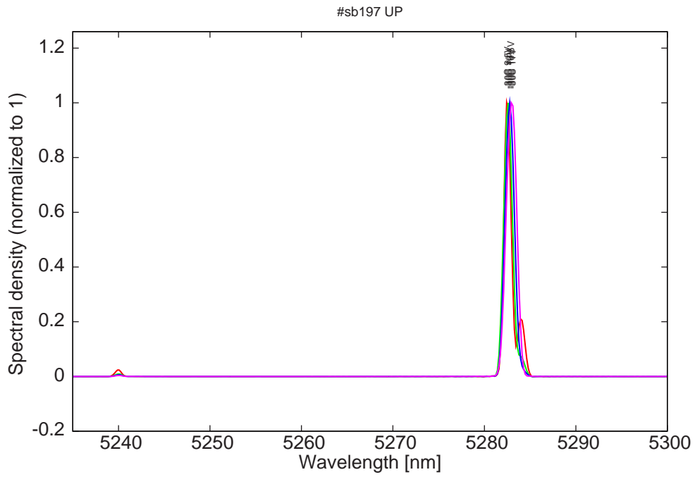
Figure 9: spectra at -30C for various LDD voltages (bimode)
