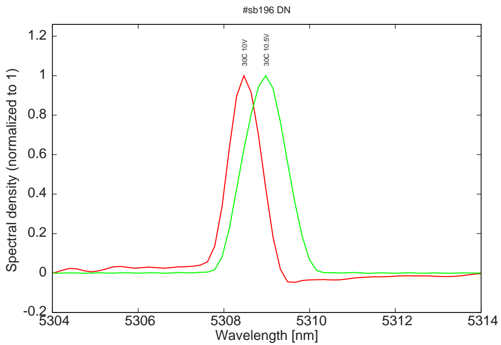
Figure 14: spectra at 30C for various LDD voltages (monomode)
