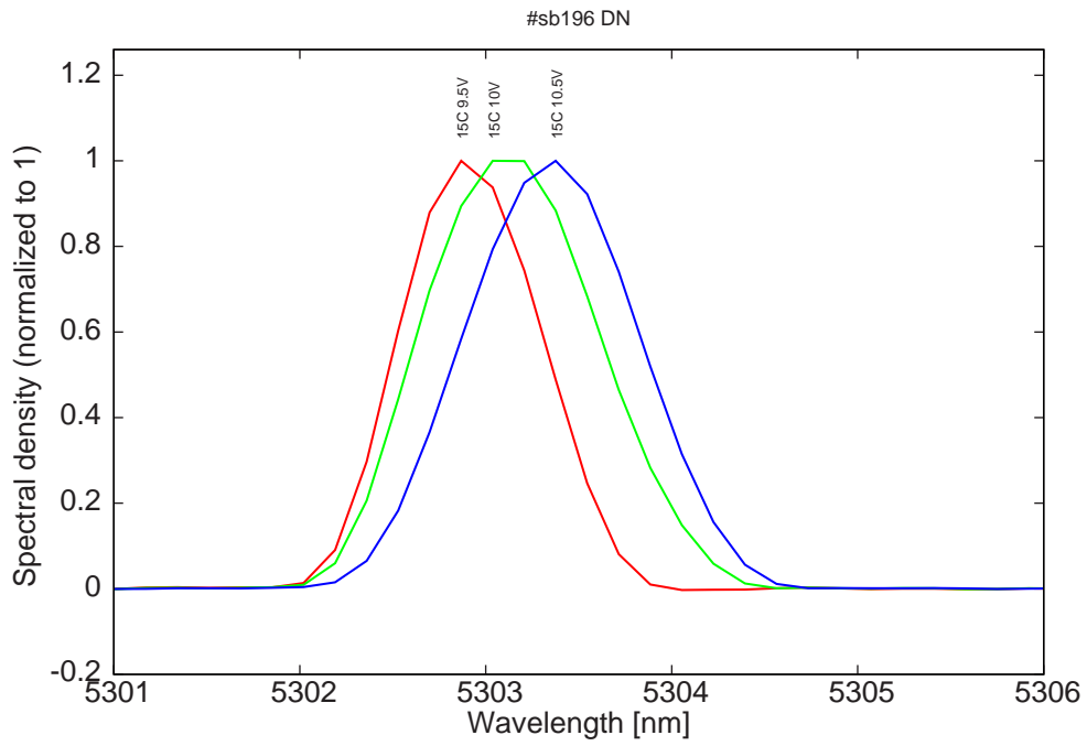
Figure 13: spectra at 15C for various LDD voltages (monomode)
