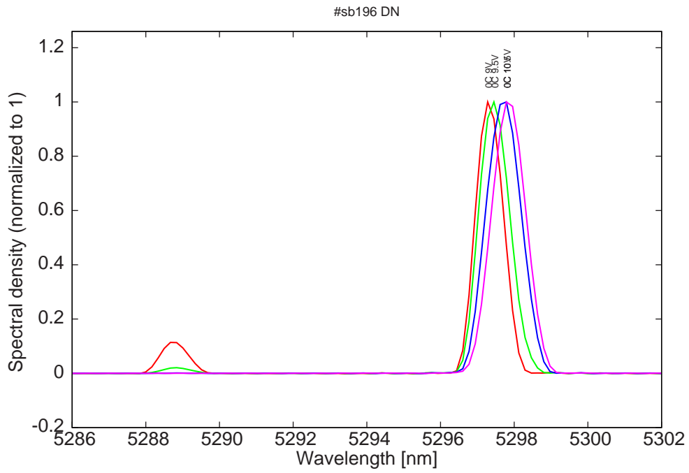
Figure 11: spectra at 0C for various LDD voltages (bimode at low LDD voltage)
