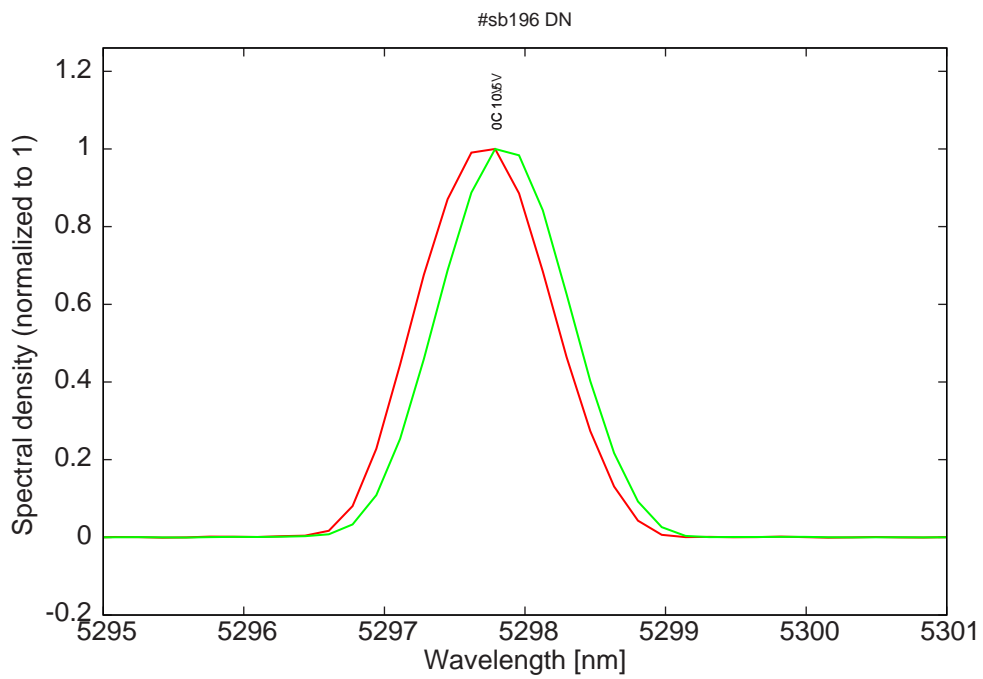
Figure 12: spectra at 0C for various LDD voltages (monomode range at high LDD voltage)
