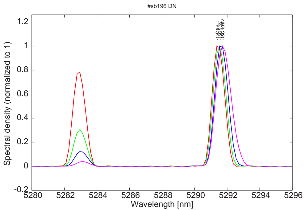
Figure 10: spectra at -15C for various LDD voltages (bimode)
