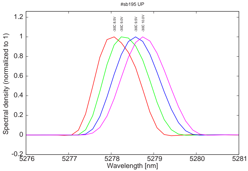
Figure 9: spectra at -30C for various LDD voltages (monomode)
