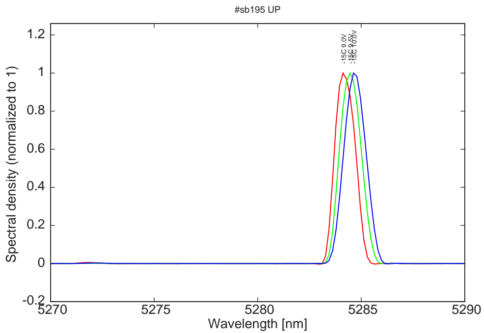
Figure 10: spectra at -15C for various LDD voltages (bimode)
