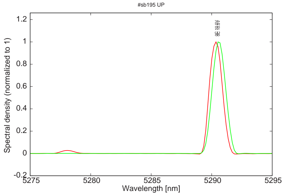
Figure 11: spectra at 0C for various LDD voltages (monomode at 10.5V)
