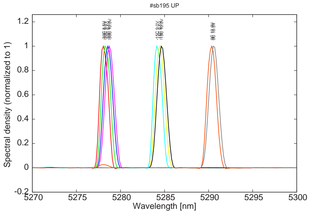
Figure 8: spectra at -30C, -15C and 0C at 2%dc for various LDD voltages
