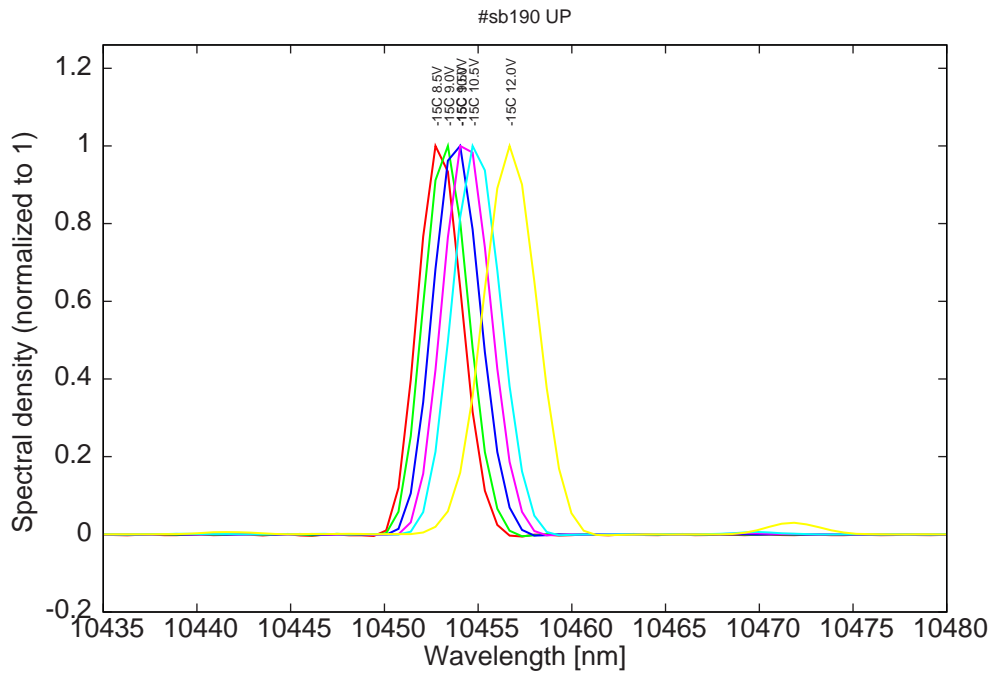
Figure 11: spectra at -15C for various LDD voltages
