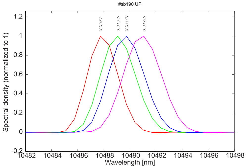
Figure 17: spectra at 30C for various LDD voltages (all monomode)
