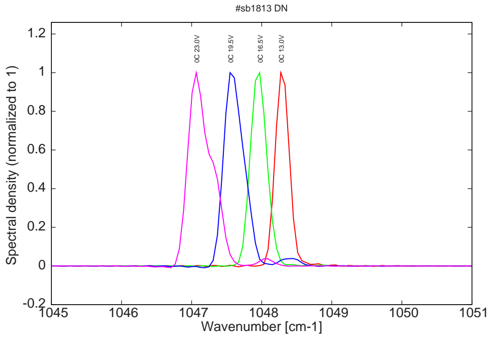
Figure 12: spectra at 0C for various LDD voltages (22ns pulses on the laser, 1.1 \mu s period)
