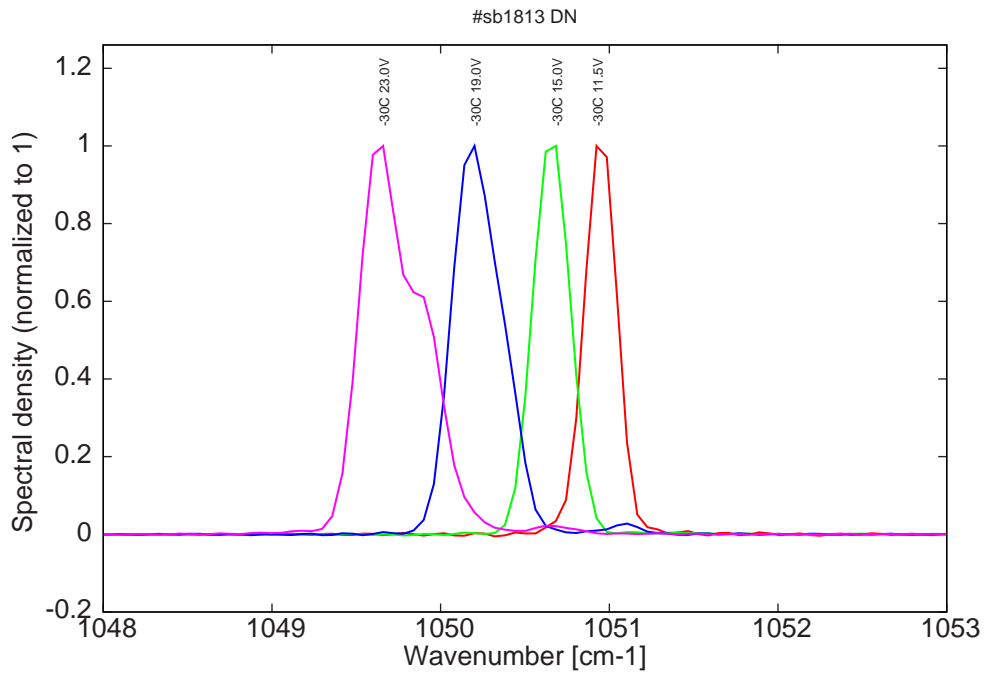
Figure 8: spectra at -30C for various LDD voltages (22ns pulses on the laser, 1.1 \mu s period)
