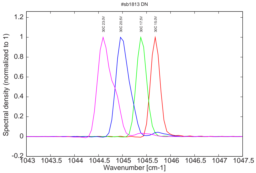
Figure 16: spectra at 30C for various LDD voltages (22ns pulses on the laser, 1.1 \mu s period)
