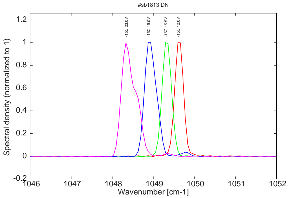
Figure 10: spectra at -15C for various LDD voltages (22ns pulses on the laser, 1.1 \mu s period)
