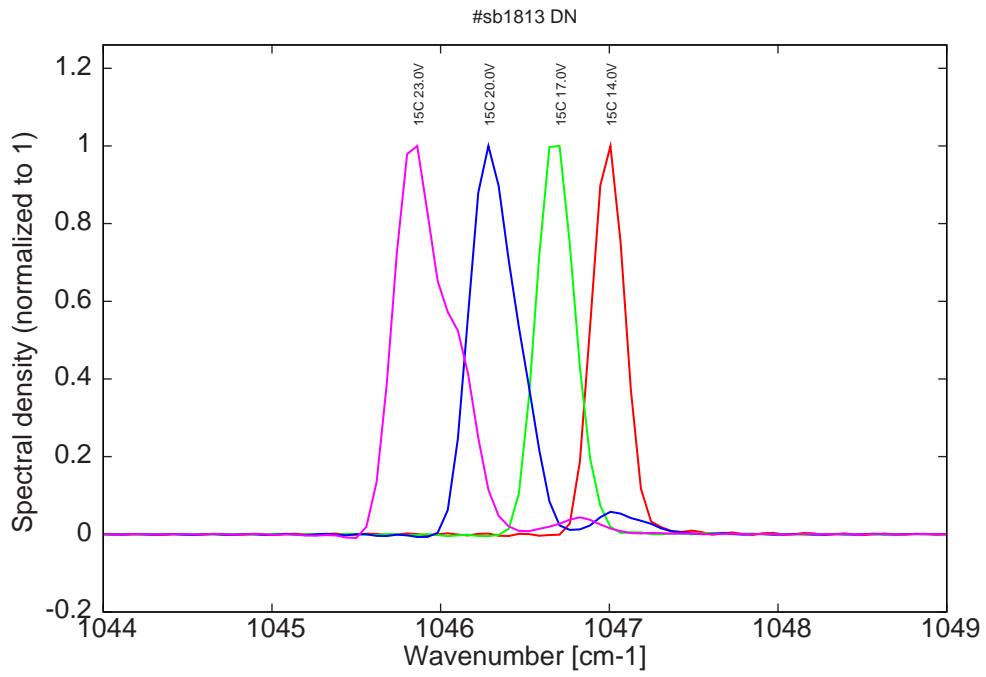
Figure 14: spectra at 15C for various LDD voltages (22ns pulses on the laser, 1.1 \mu s period)
