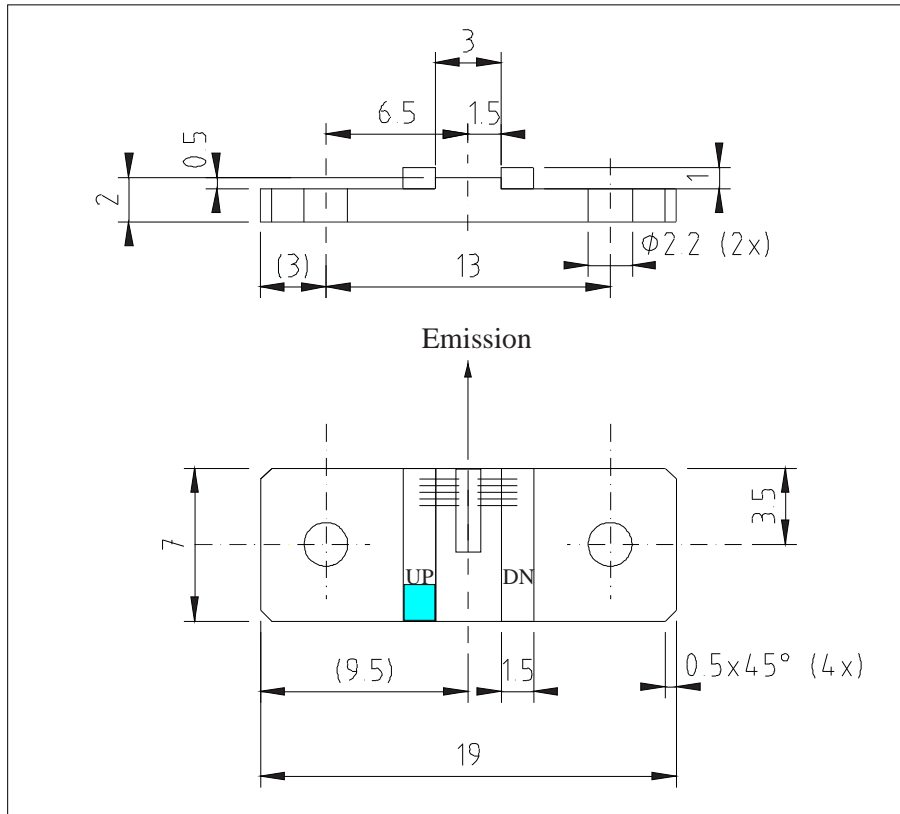
Figure 1: Support mounting for #sb1793 UP (please note that the laser is connected to the UP pad drawn in blue)
