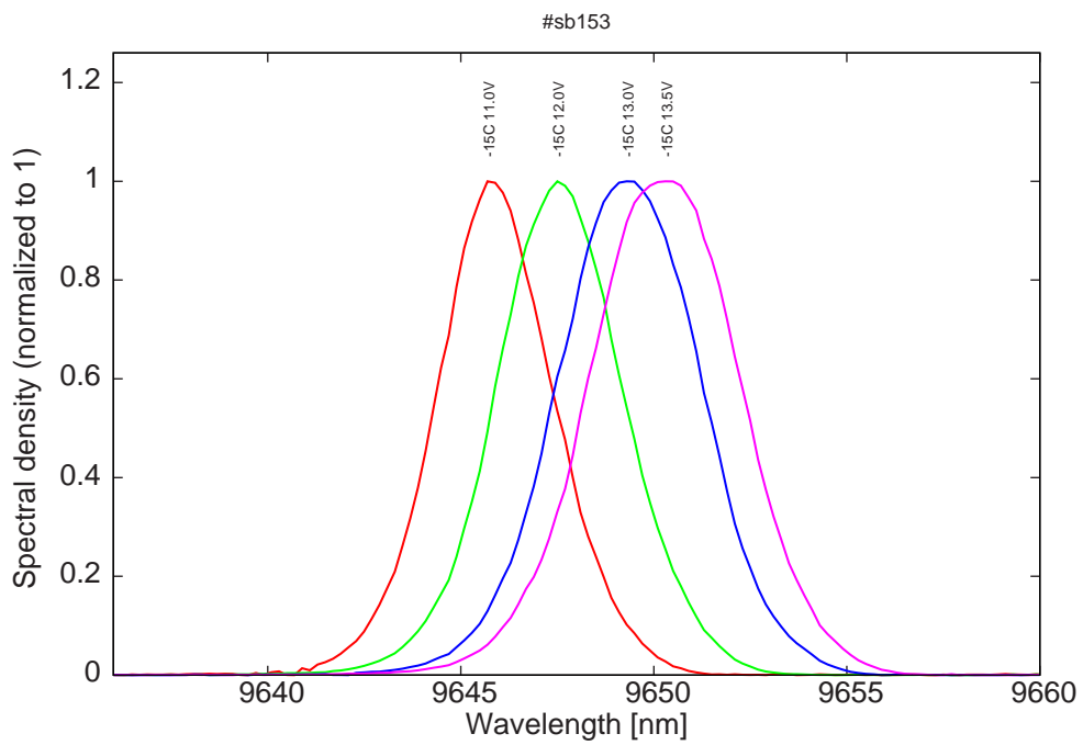
Figure 8: spectra at -15C for various LDD voltage
