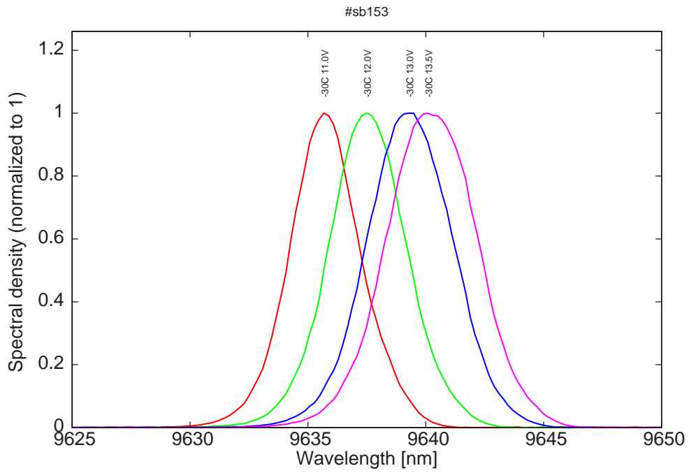
Figure 7: spectra at -30C for various LDD voltage
