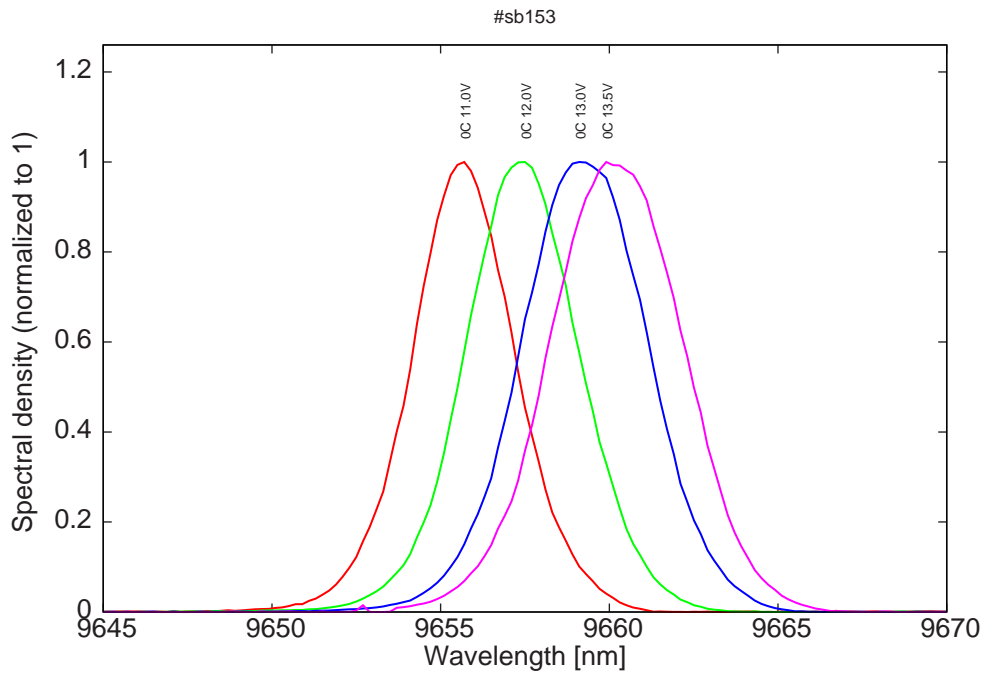
Figure 9: spectra at 0C for various LDD voltage
