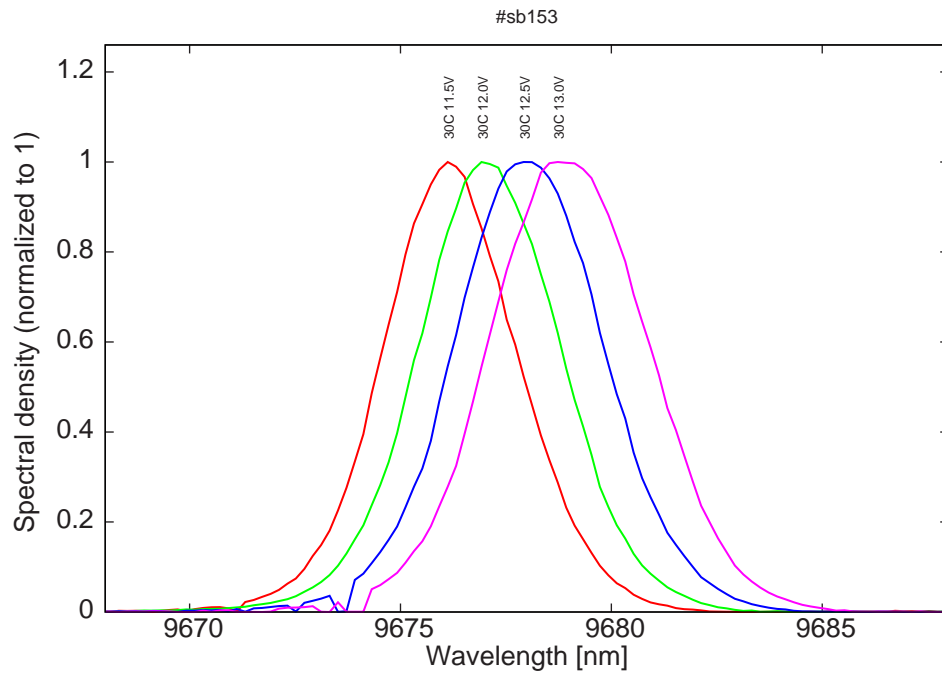
Figure 11: spectra at 30C for various LDD voltage
