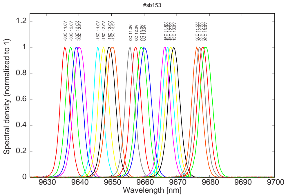
Figure 6: spectra at -30C, -15C, 0C, 15C and 30C at 2%dc for various LDD voltage
