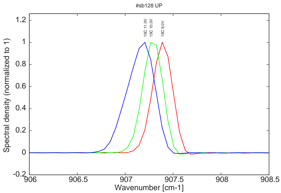
Figure 15: spectra at 15C at 2% dc for various LDD voltages (monomode range)
