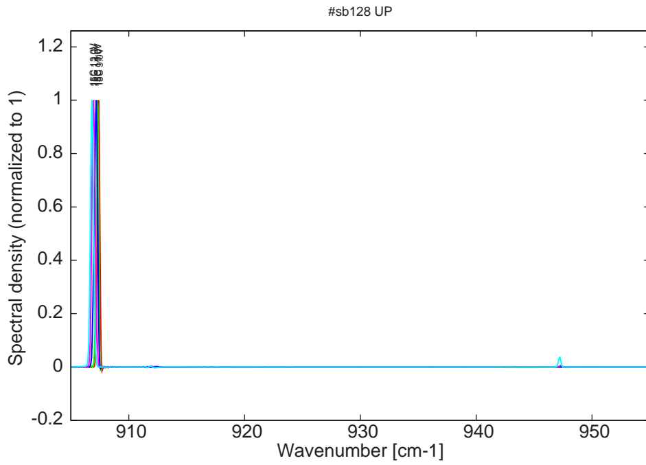
Figure 14: spectra at 15C at 2% dc for various LDD voltages
