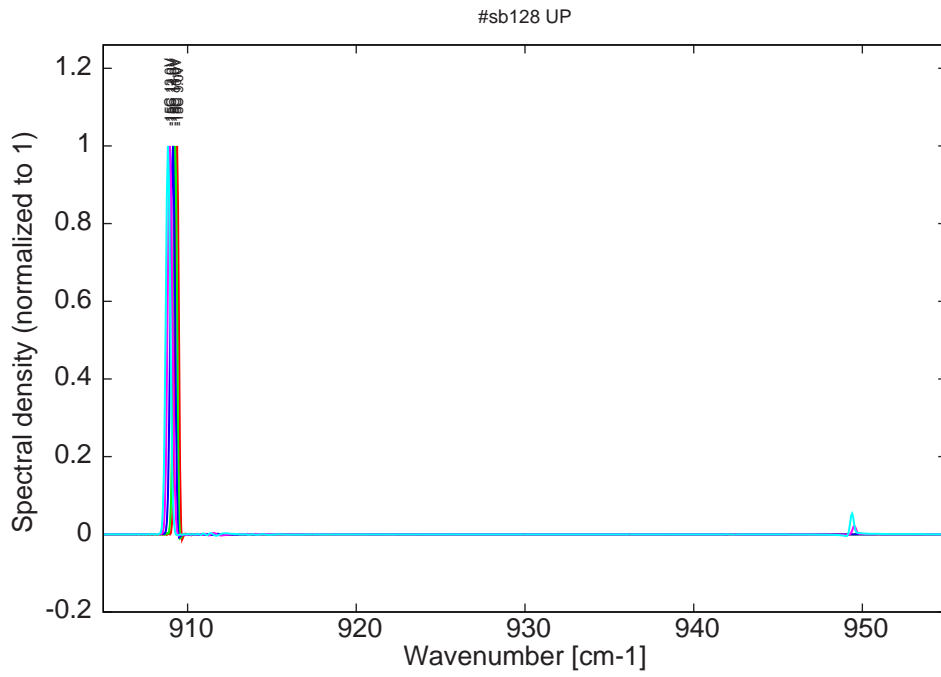
Figure 10: spectra at -15C at 2% dc for various LDD voltages
