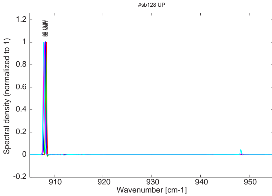
Figure 12: spectra at 0C at 2% dc for various LDD voltages
