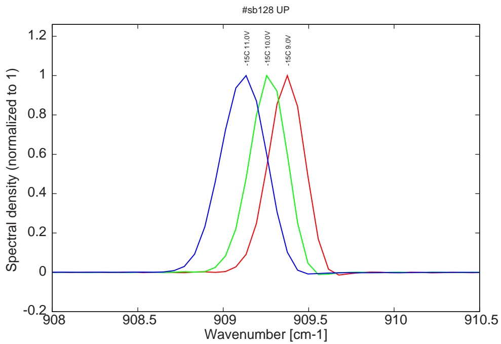
Figure 11: spectra at -15C at 2% dc for various LDD voltages (monomode range)
