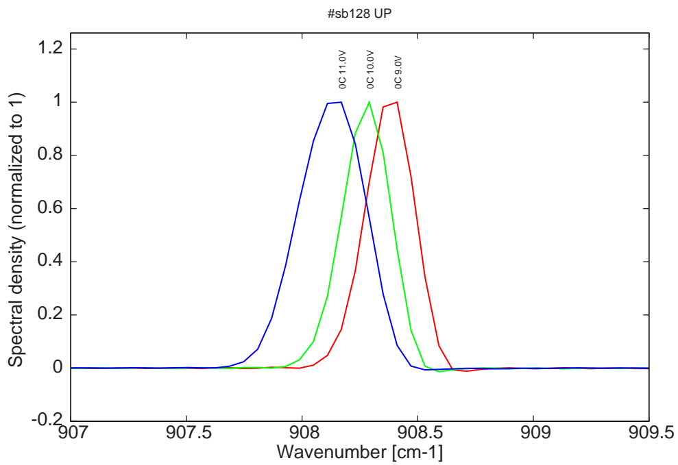
Figure 13: spectra at 0C at 2% dc for various LDD voltages (monomode range)
