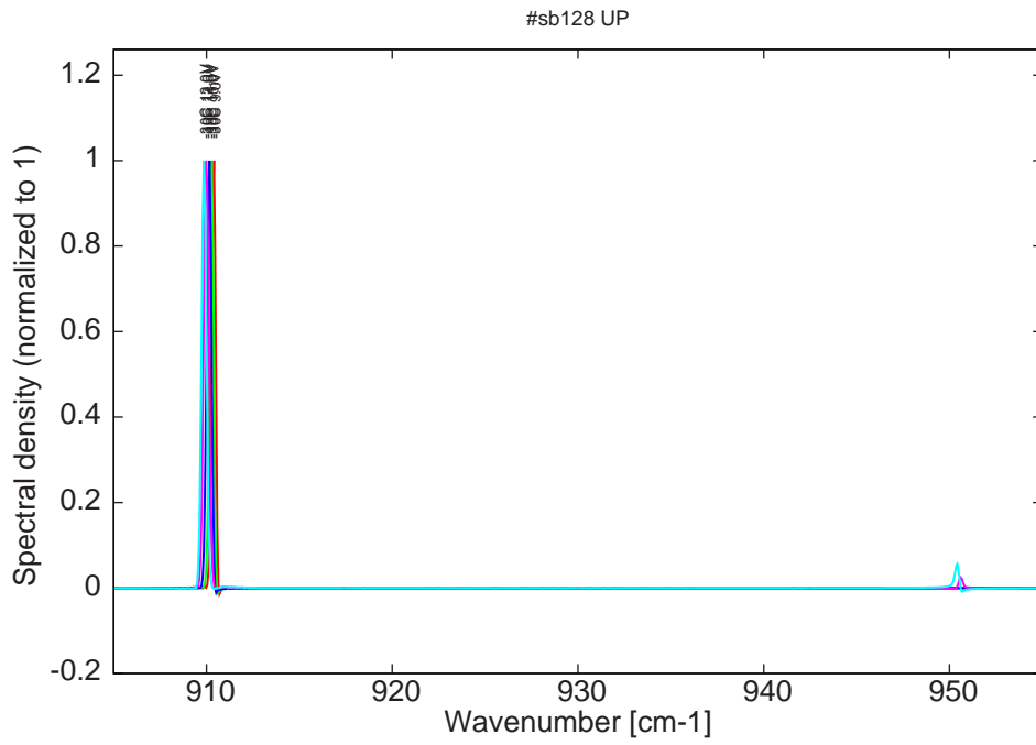
Figure 8: spectra at -30C at 2% dc for various LDD voltages
