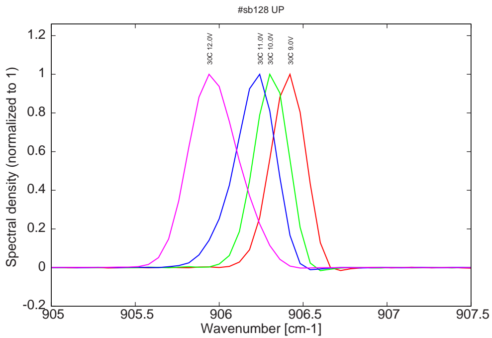
Figure 17: spectra at 30C at 2% dc for various LDD voltages (monomode range)
