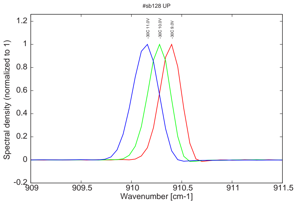
Figure 9: spectra at -30C at 2% dc for various LDD voltages (monomode range)
