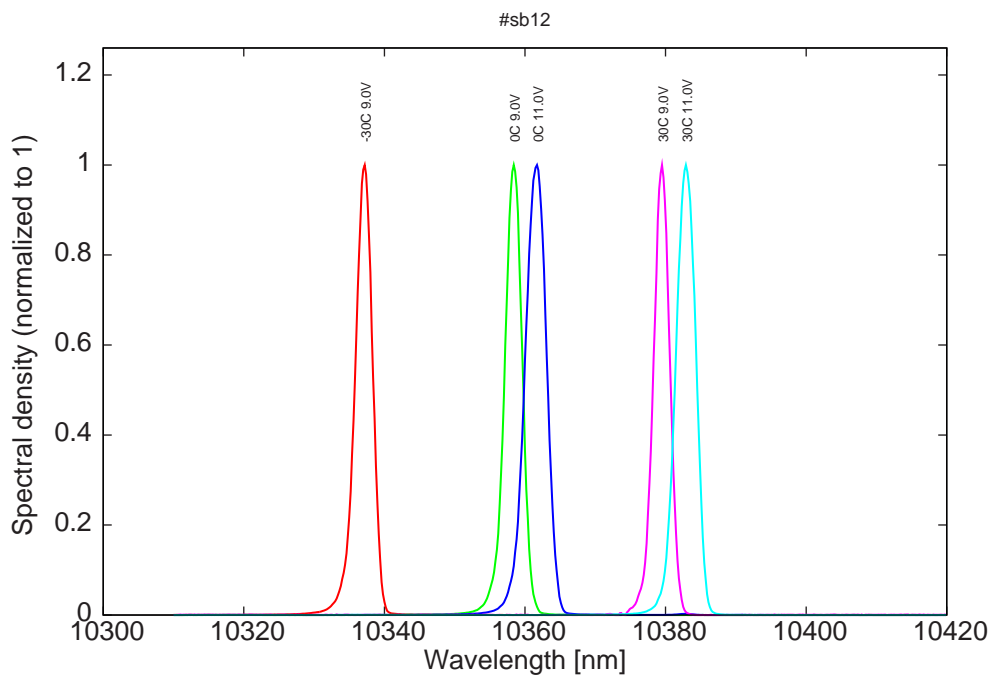
Figure 8: monomode spectra for various temperatures and lower LDD voltages
