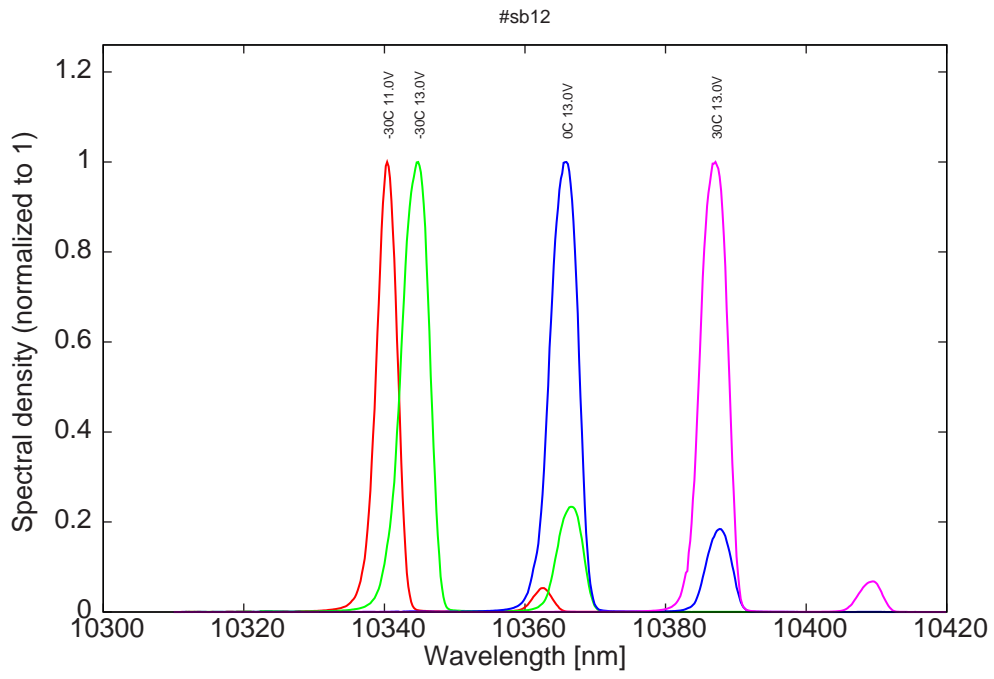
Figure 9: bimode spectra for various temperatures and higher LDD voltages
