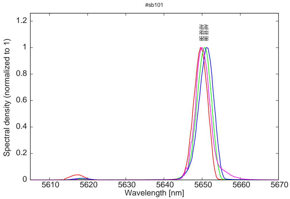
Figure 10: spectra at 0C for various LDD voltages (bimode)
