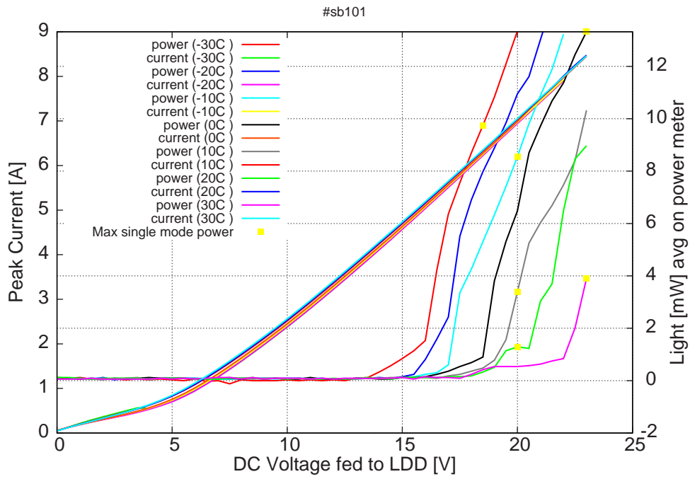
Figure 4: peak current and avg power vs LDD voltage (the solid squares indicate the maximum singlemode emitted power)
