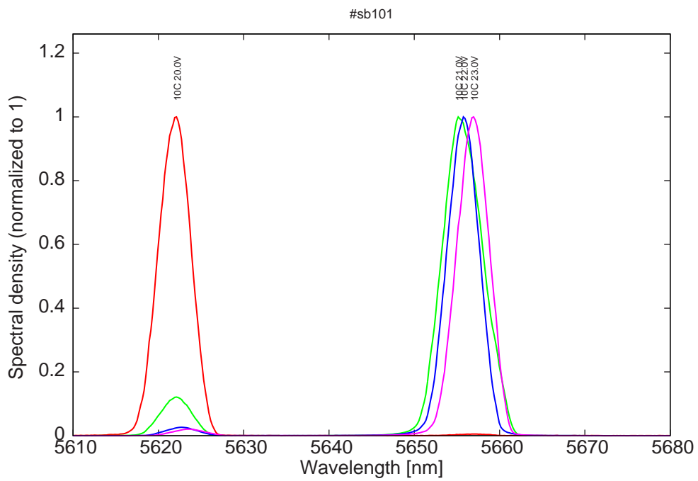
Figure 11: spectra at 10C for various LDD voltages (bimode)
