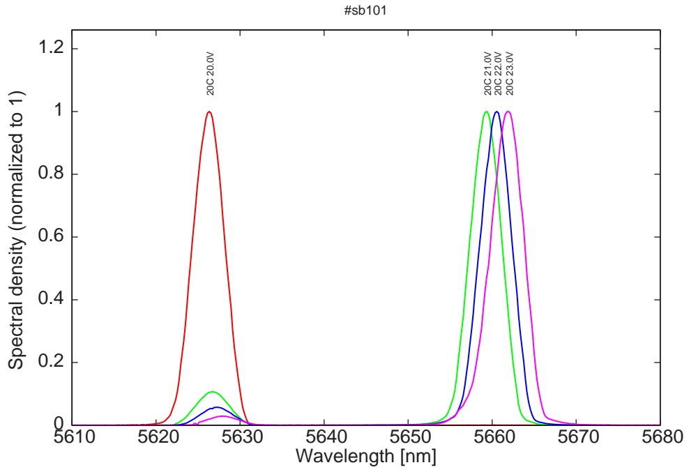
Figure 12: spectra at 20C for various LDD voltages (mono at threshold)
