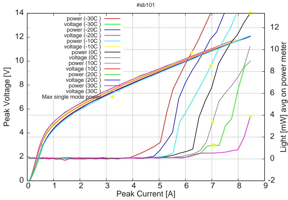
Figure 2: peak voltage and avg power vs peak current (the solid squares indicate the maximum singlemode emitted power)
