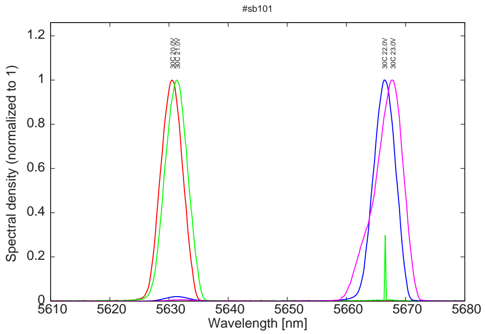
Figure 13: spectra at 30C for various LDD voltages (mono at threshold)
