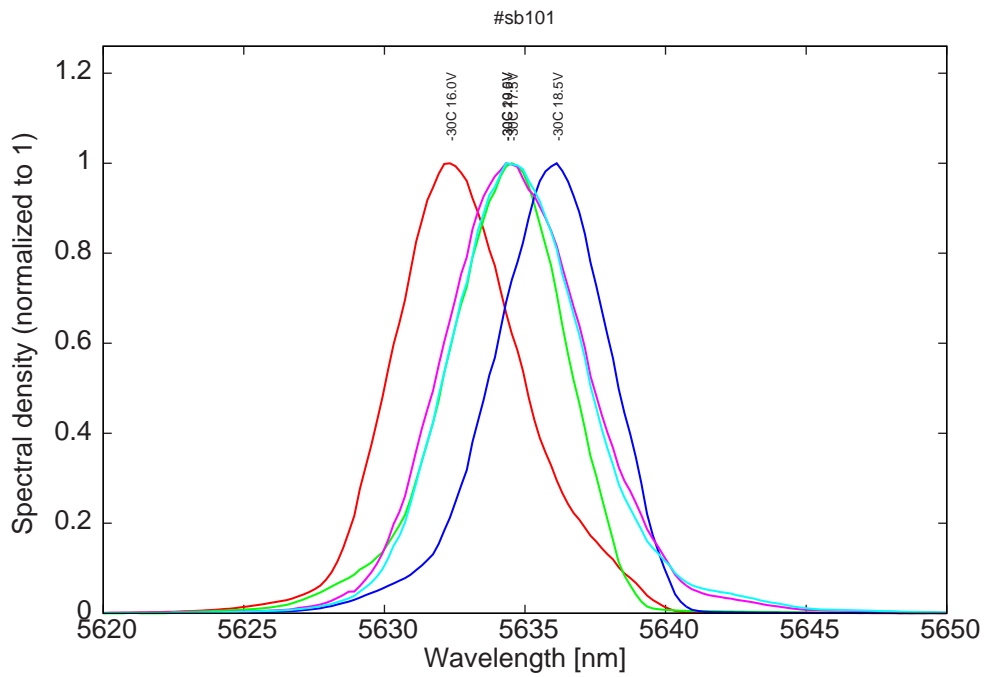
Figure 7: spectra at -30C for various LDD voltages (mode jumping at 19.5V)
