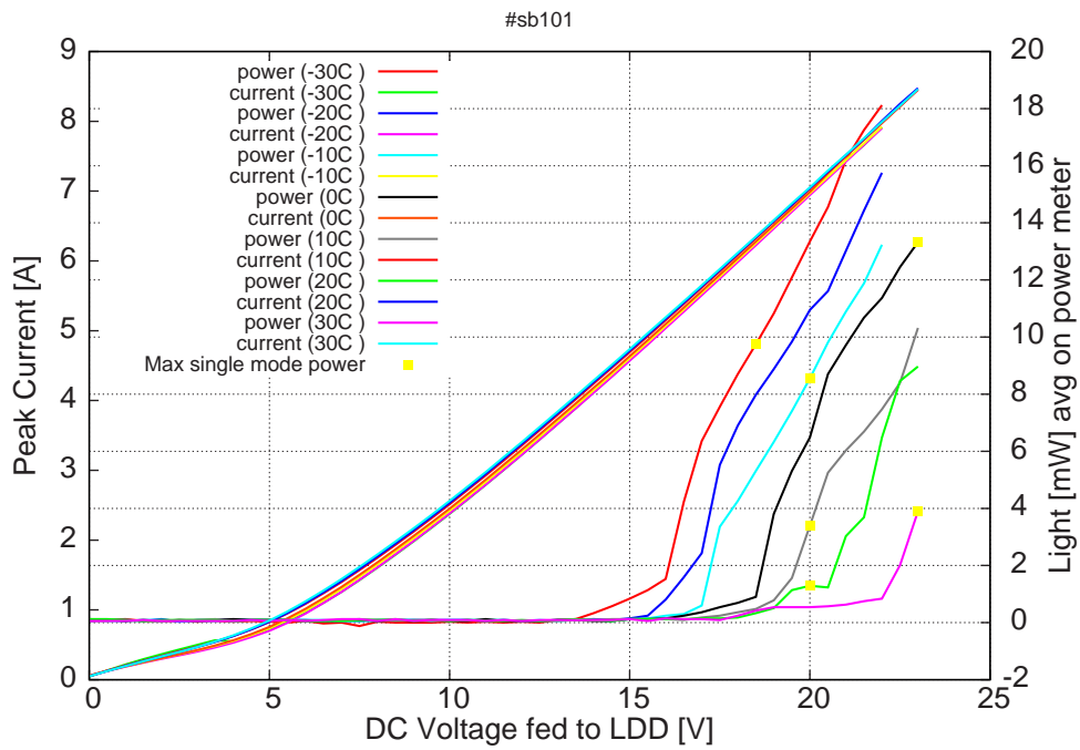
Figure 5: peak current and avg power vs LDD voltage (including the multimode region)
