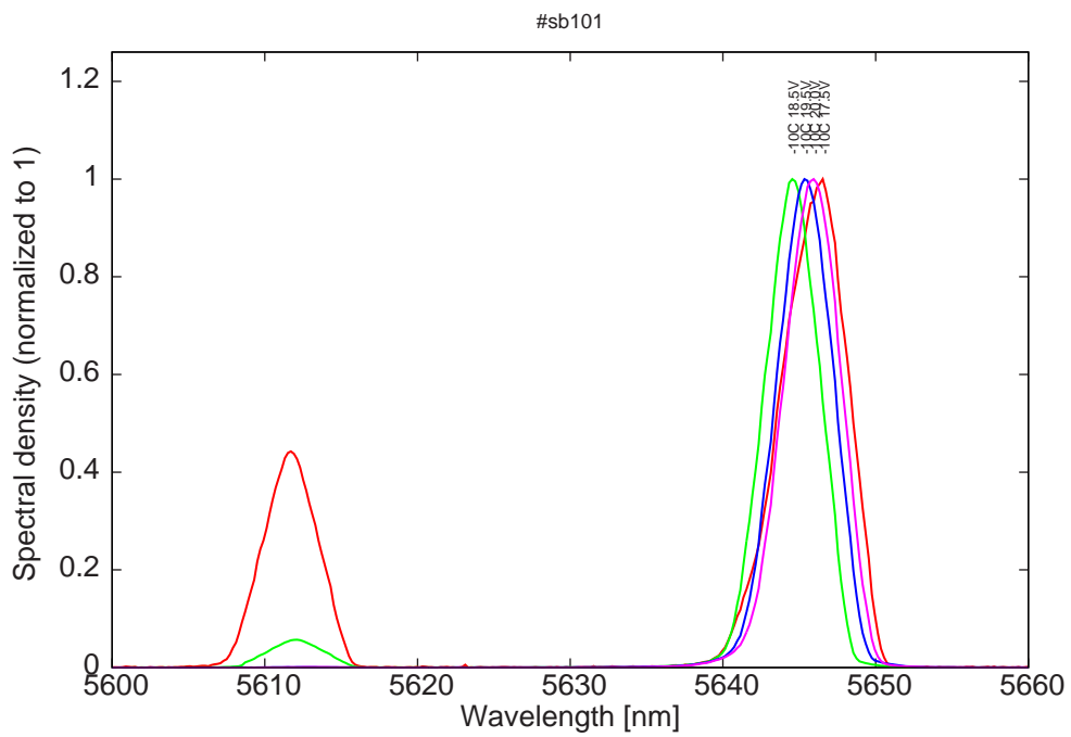
Figure 9: spectra at -10C for various LDD voltages
