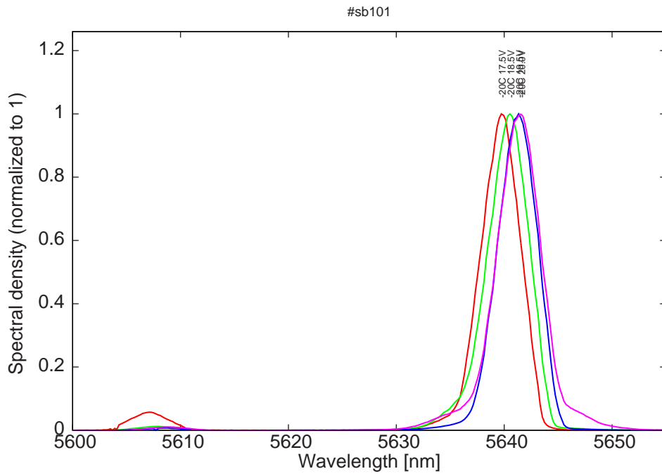
Figure 8: spectra at -20C for various LDD voltages (bimode)
