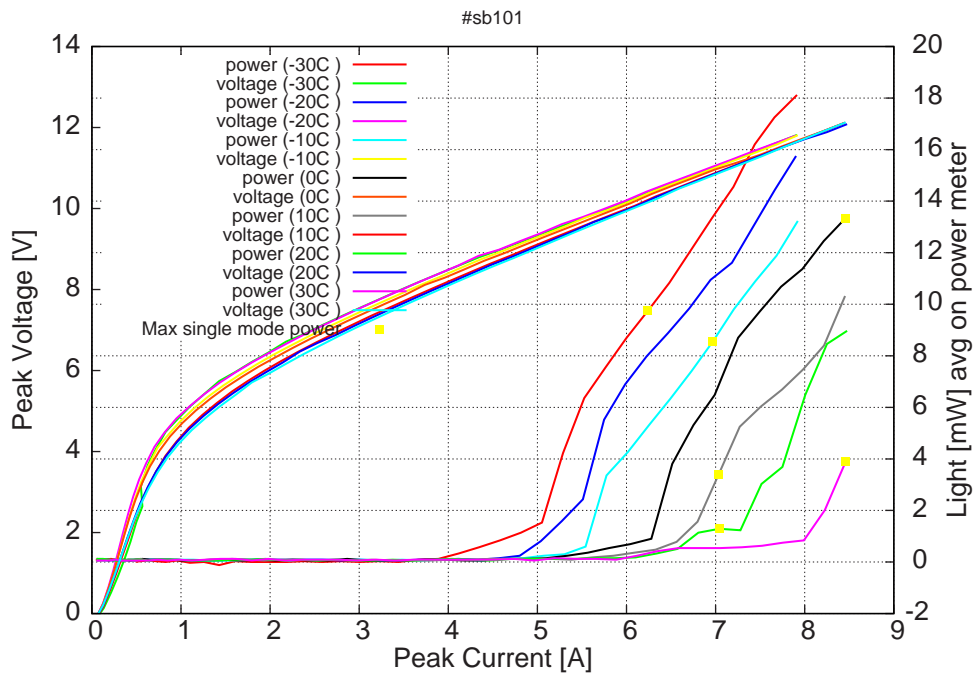
Figure 3: peak voltage and avg power vs peak current (including the multimode region)
