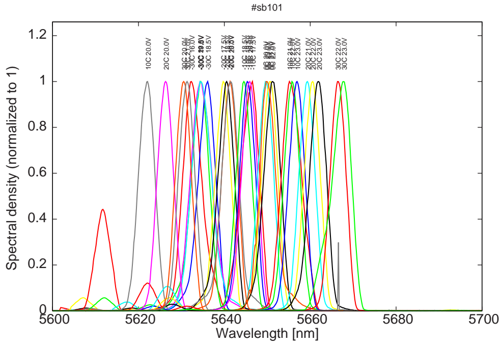
Figure 6: spectra from -30C to 30C for various LDD voltages
