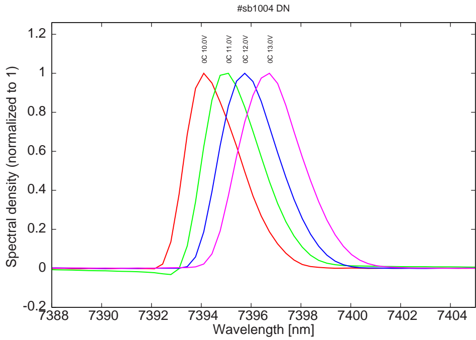
Figure 11: spectra at 0C for various LDD voltages
