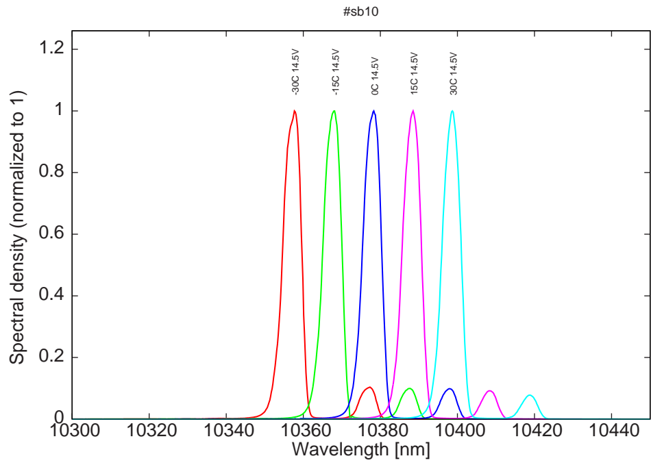
Figure 9: bimode spectra for various temperatures and high LDD voltages
