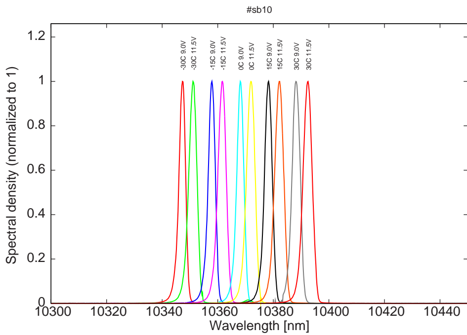
Figure 8: monomode spectra for various temperatures and lower LDD voltages
