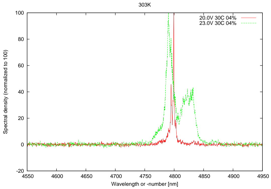
Figure 4: spectra at 30C at 4% dc at 20V and 23V on LDD (corresponding respectively to an output power of 11mW and 61mW)
