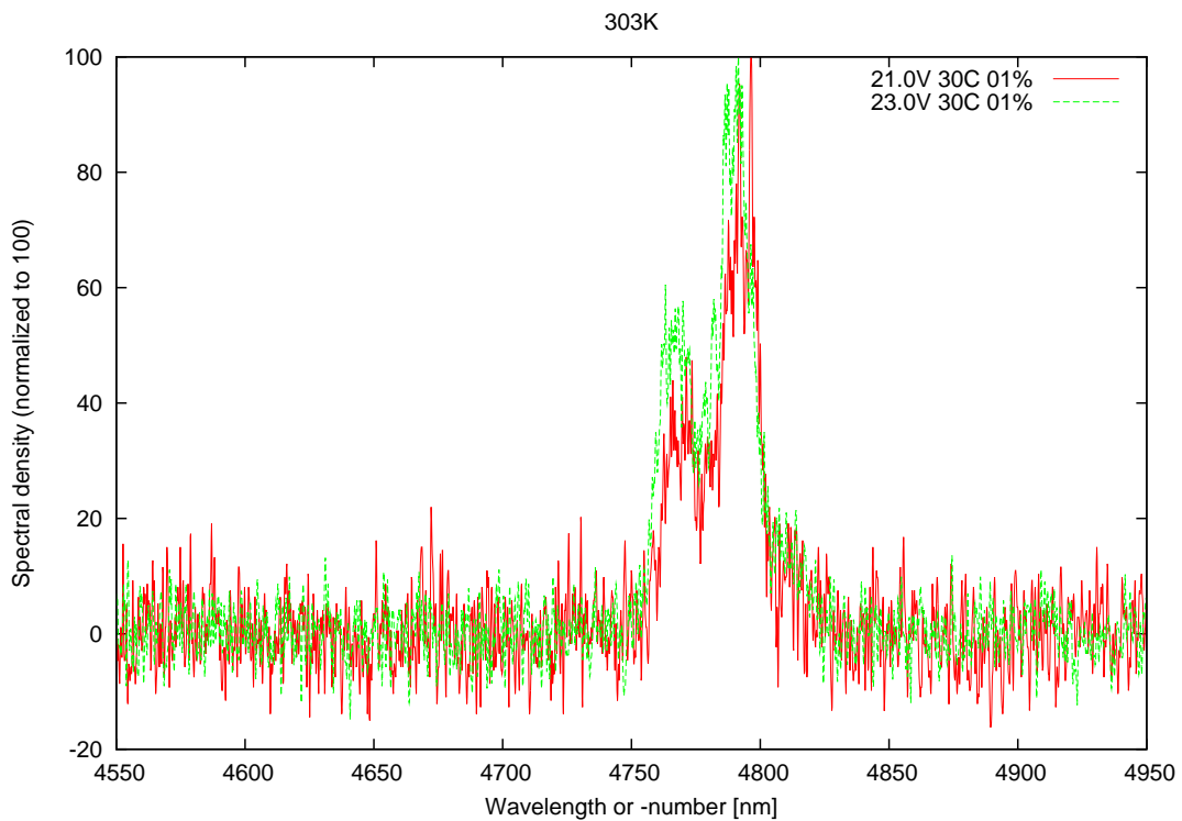
Figure 3: spectra at 30C at 1% dc at 21V and 23V on LDD (corresponding respectively to an output power of 7mW and 18mW)
